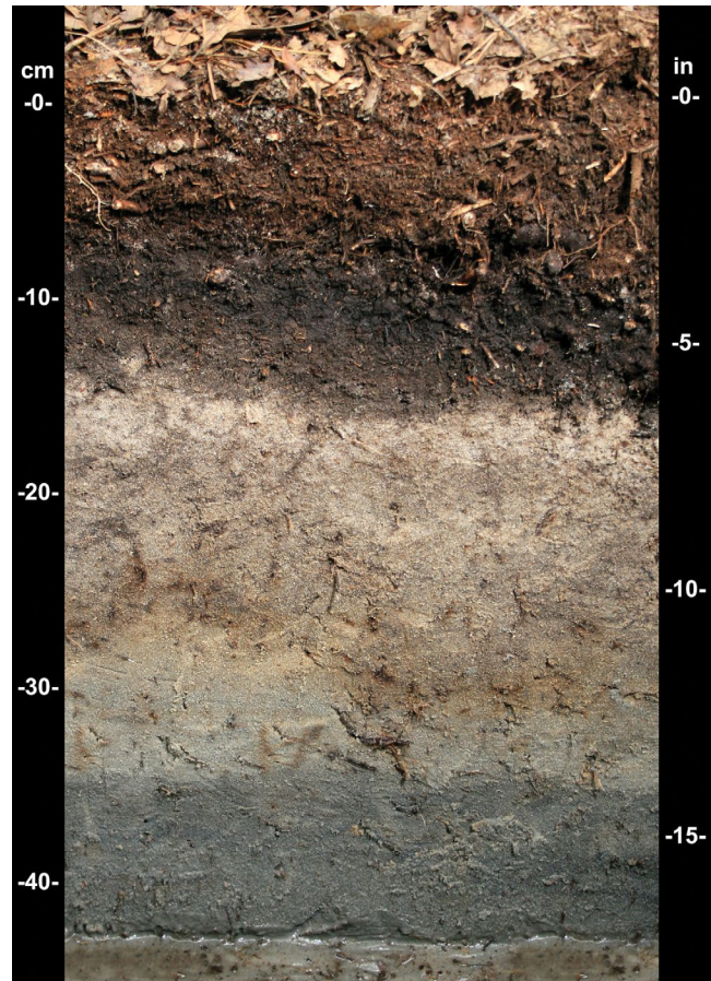
Figure 2.— The soil profile above consists of an 8 cm (3.14 inches) layer of peat and/or mucky peat underlain by a 1 cm (0.4 inches) layer of muck. The remaining soil layers are sandy soil material. In LRRs R, W, X, and Y, observations would begin below the peat, mucky peat, and muck layers (9 cm). In LRRs F, G, H, and M, observations would start at the actual soil surface. In all remaining LRRs, observations would begin at the muck surface (8 cm).
