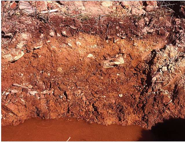
Figure 40.—Indicator F21 (Red Parent Material). This indicator should be used only in areas of red parent material that is resistant to reduction. Not all red soils formed in red parent material.
