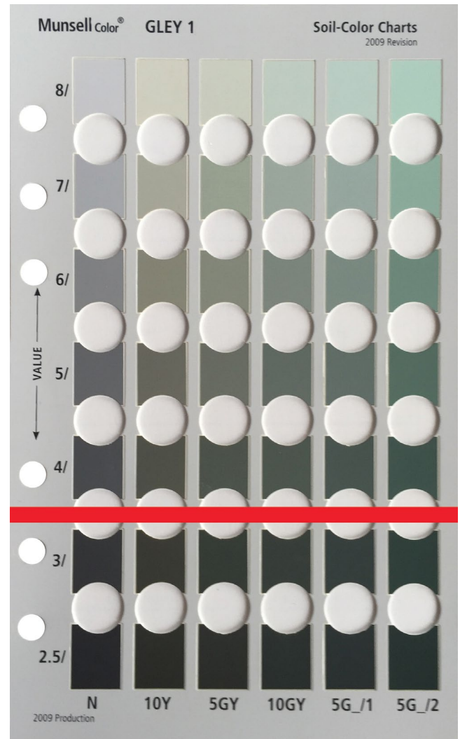
Figure 50. —A gleyed matrix must have the colors on one of the two pages showing gleyed colors in the Munsell Soil Color Book. Values are 4 or more (above the red line).
