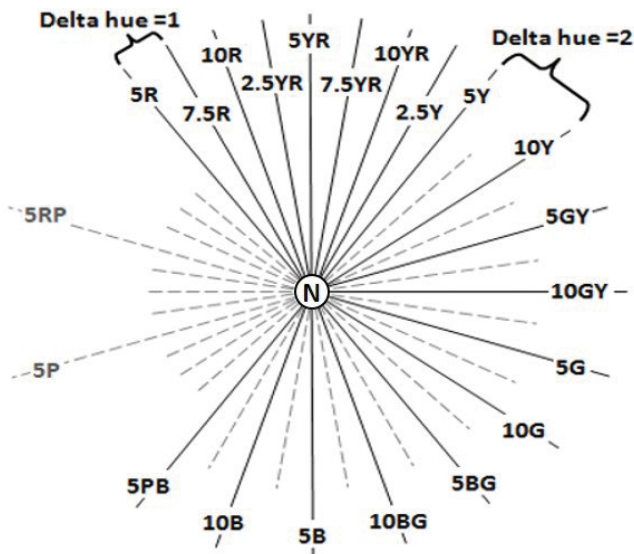
Figure 48.—Relationships among the hues of the Munsell Color System. Solid lines represent hues contained in the Munsell Soil Color Charts (2009). Dotted lines represent all other possible 2.5-unit steps. Moving from one hue line to the adjacent hue line represents a delta hue of 1 (2.5 units). Moving from hue N to any other hue the delta hue is 1. Adapted from the Soil Survey Manual (Soil Survey Staff, 1993).
