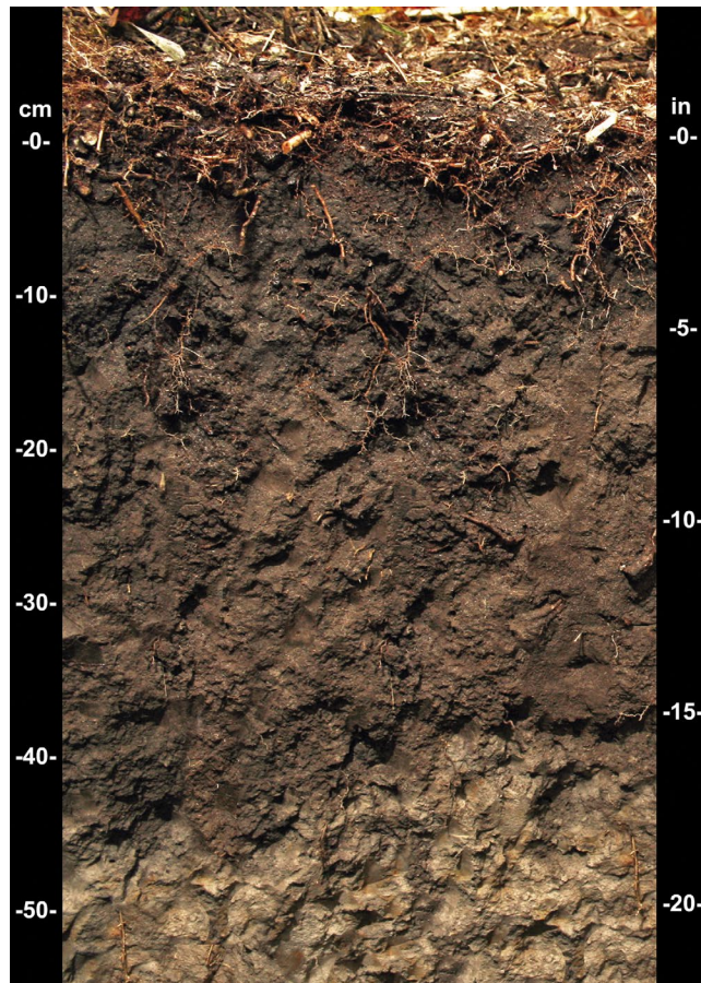
Figure 37.—Indicator F13 (Umbric Surface). This soil has an umbric surface horizon about 44 cm thick. It meets the requirements not only of indicator F13 but also of indicators A7 (5 cm Mucky Mineral) and A12 (Thick Dark Surface).
