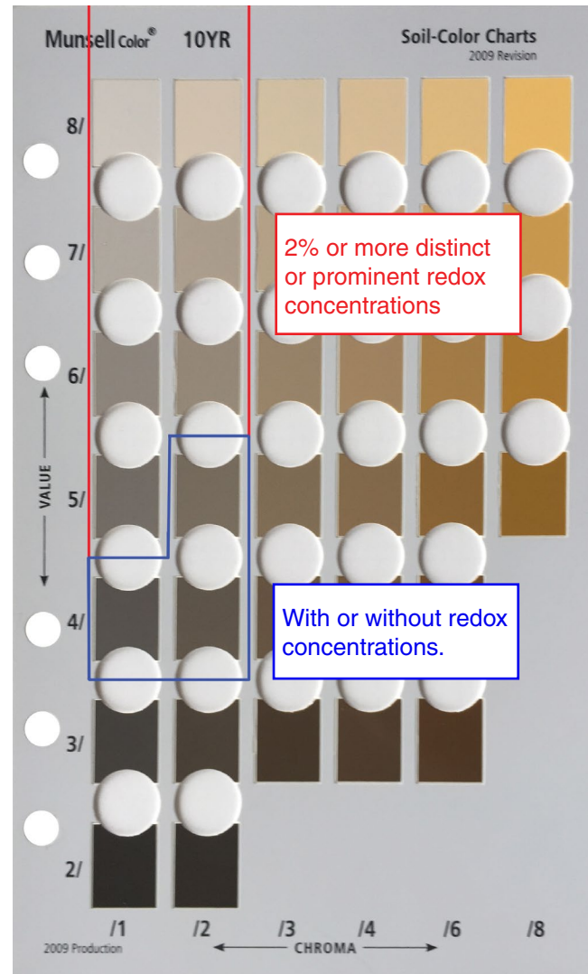
Figure 44.—Illustration of values and chromas that require 2 percent or more distinct or prominent redox concentrations and those that do not, for hue 10YR, to meet the definition of a depleted matrix. Due to inaccurate color reproduction, do not use this page to determine soil colors in the field. Background image from the Munsell Soil Color Charts reprinted courtesy of Munsell Color Services Lab, a part of X-Rite, Inc. (Xrite 2009).
