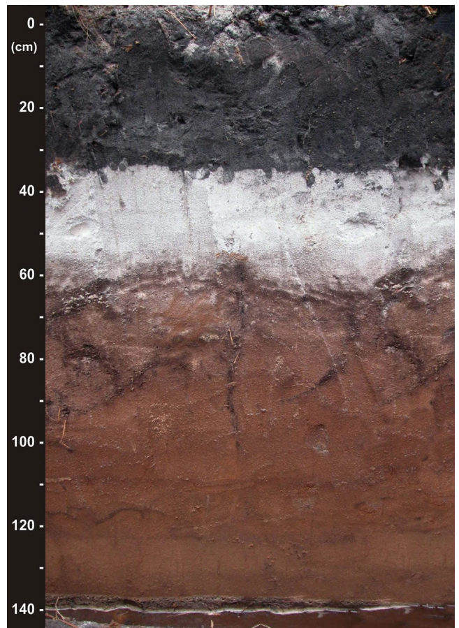
Figure 47. —A soil profile with an albic (white) E horizon between depths of about 35 and 60 cm. The white color results from loss of iron through weathering.
