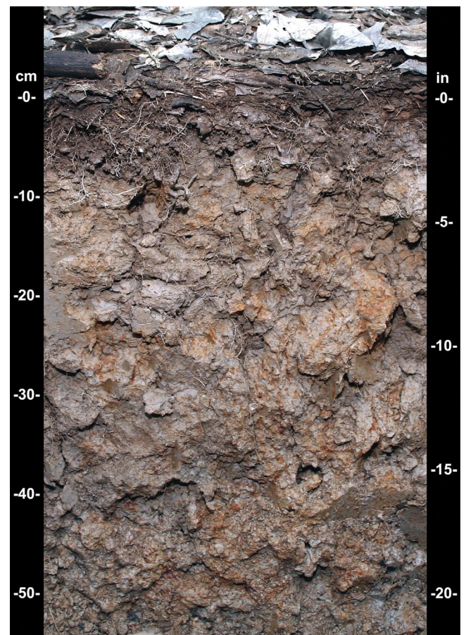
Figure 29.—Indicator F3 (Depleted Matrix). This soil has value of 4 or more and chroma of 2 or less and redox concentrations starting at a depth of 8 cm. Since the depleted matrix starts at a depth of \leq 15 cm from the soil surface, the minimum thickness requirement is only 5 cm.
