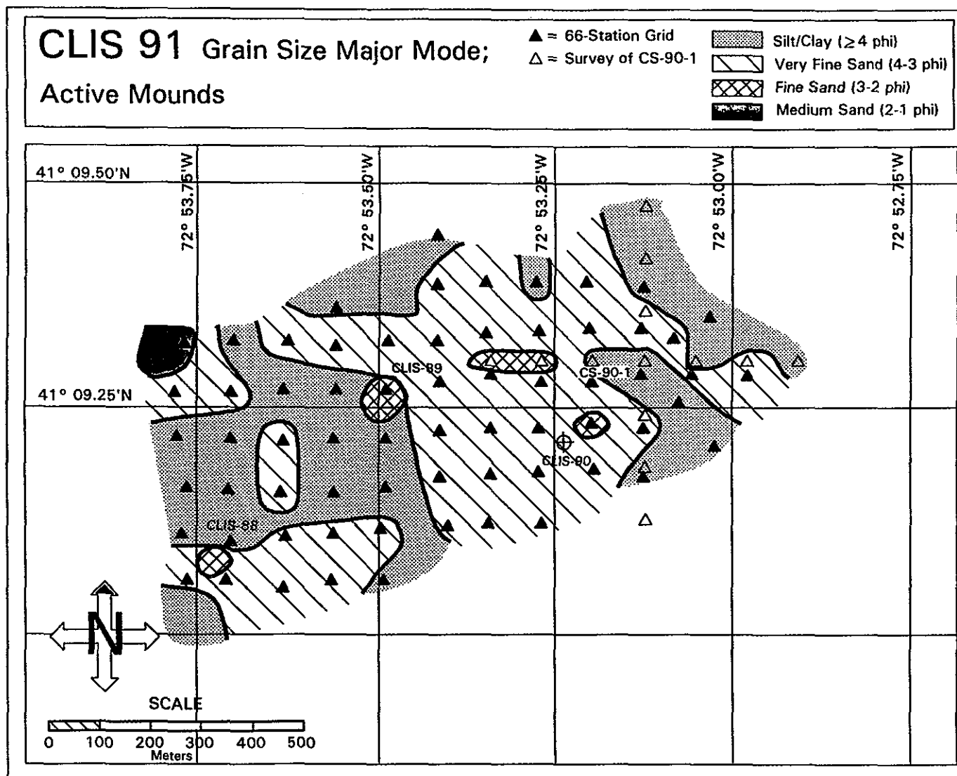
Figure 3-5. Map of sediment grain size major mode (in phi units) at CLIS active disposal mounds, June 1991
