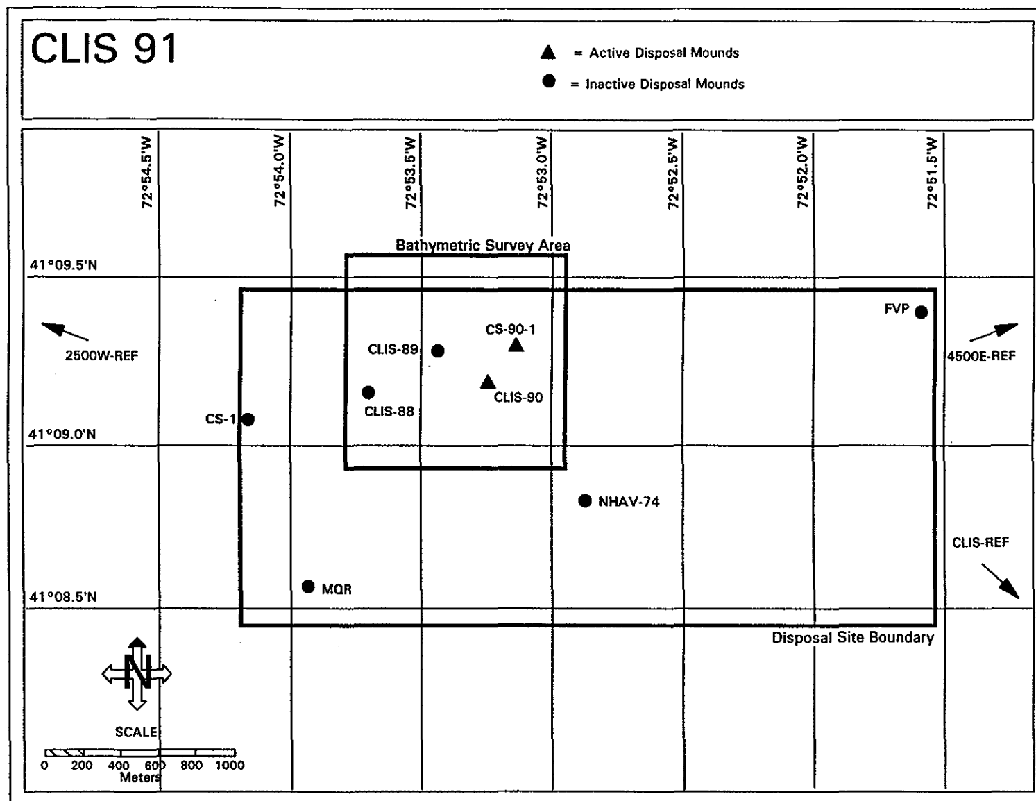
Figure 1-2. Locations of the surveyed active and inactive disposal mounds and the bathymetric survey area at CLIS, June 1991
