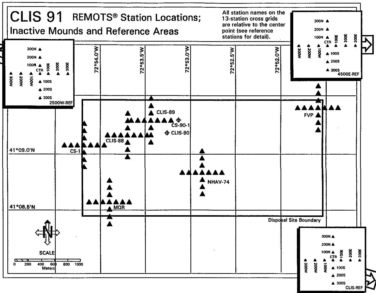
Figure 2-1. Locations and designations of REMOTS® stations over inactive mounds and reference areas surveyed at CLIS, June 1991
