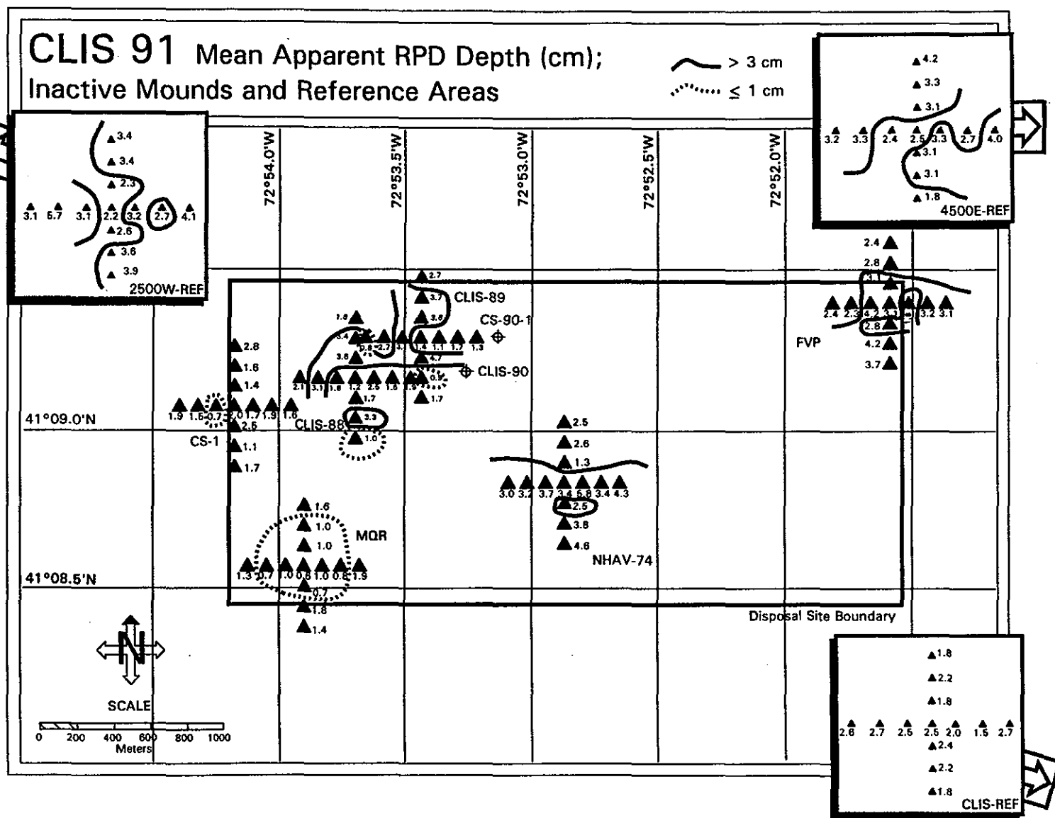
Figure 3-15. The mapped distribution of apparent RPD depths (cm) at CLIS inactive disposal mounds and reference areas, June 1991
