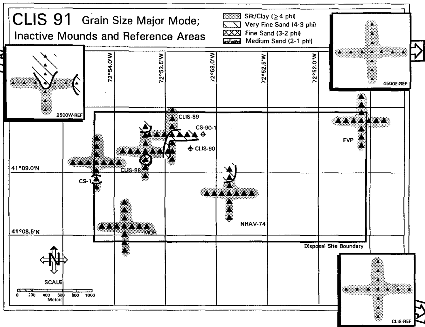
Figure 3-6. Map of sediment grain size major mode (in phi units) at CLIS inactive disposal mounds and reference areas, June 1991
