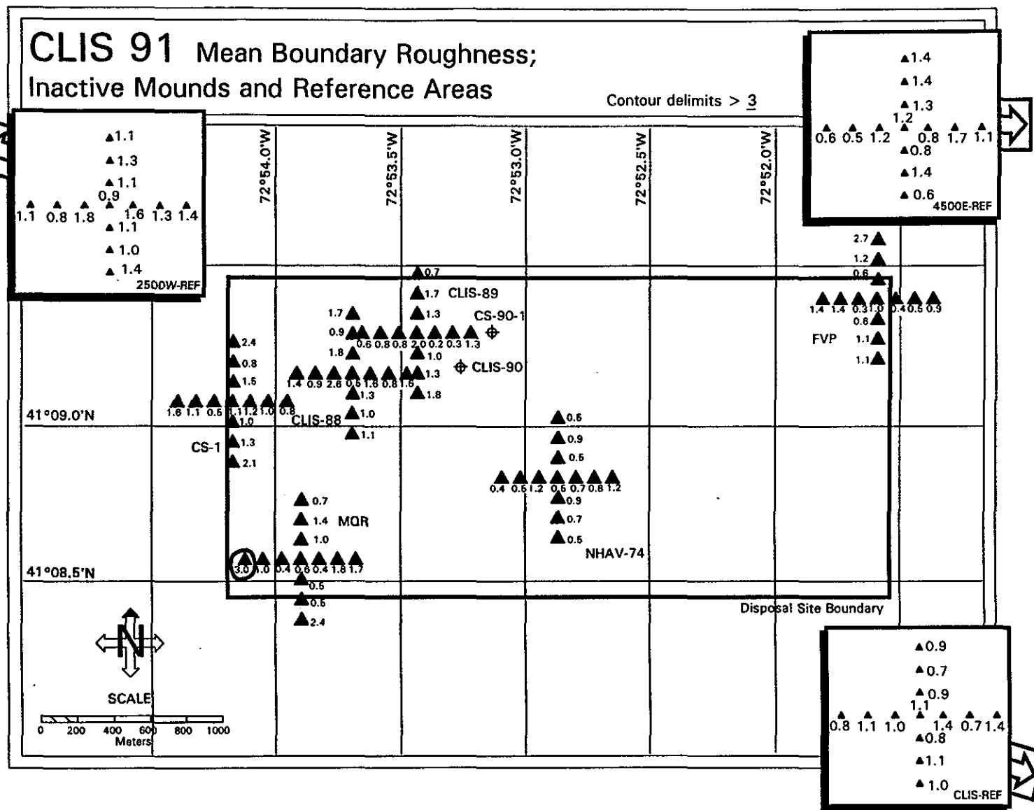
Figure 3-12. Map of mean small-scale surface boundary roughness values at CLIS inactive mounds and reference areas, June 1991
