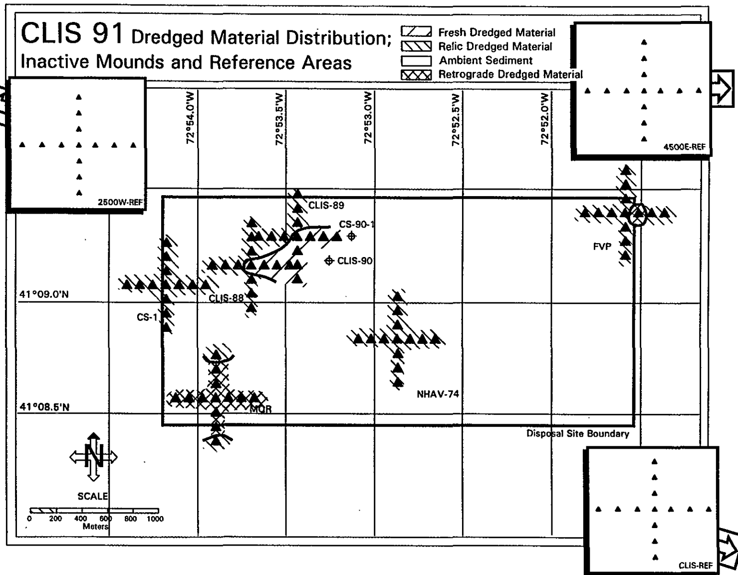
Figure 3-9. Distribution of dredged material at CLIS inactive mounds and reference areas, June 1991
