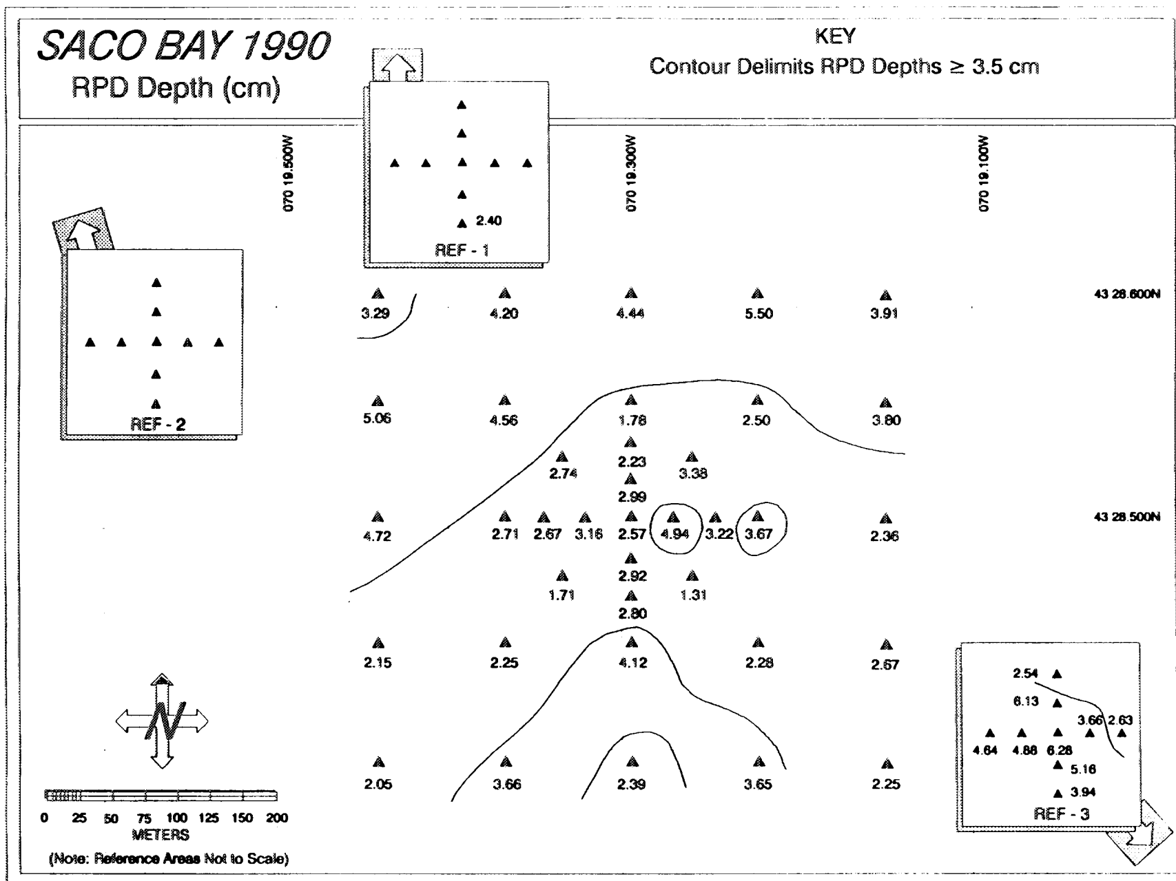
Figure 3-8. Mapped distribution of mean apparent RPD depths at Saco Bay Disposal Site and reference stations, May 1990.
