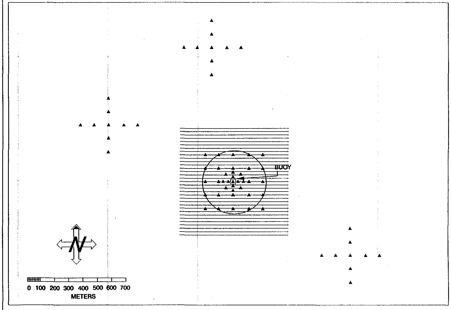
Figure 2-1. Bathymetric survey lanes, buoy position, and relative position of REMOTS® grid and reference stations. Circle indicates disposal site boundary.
