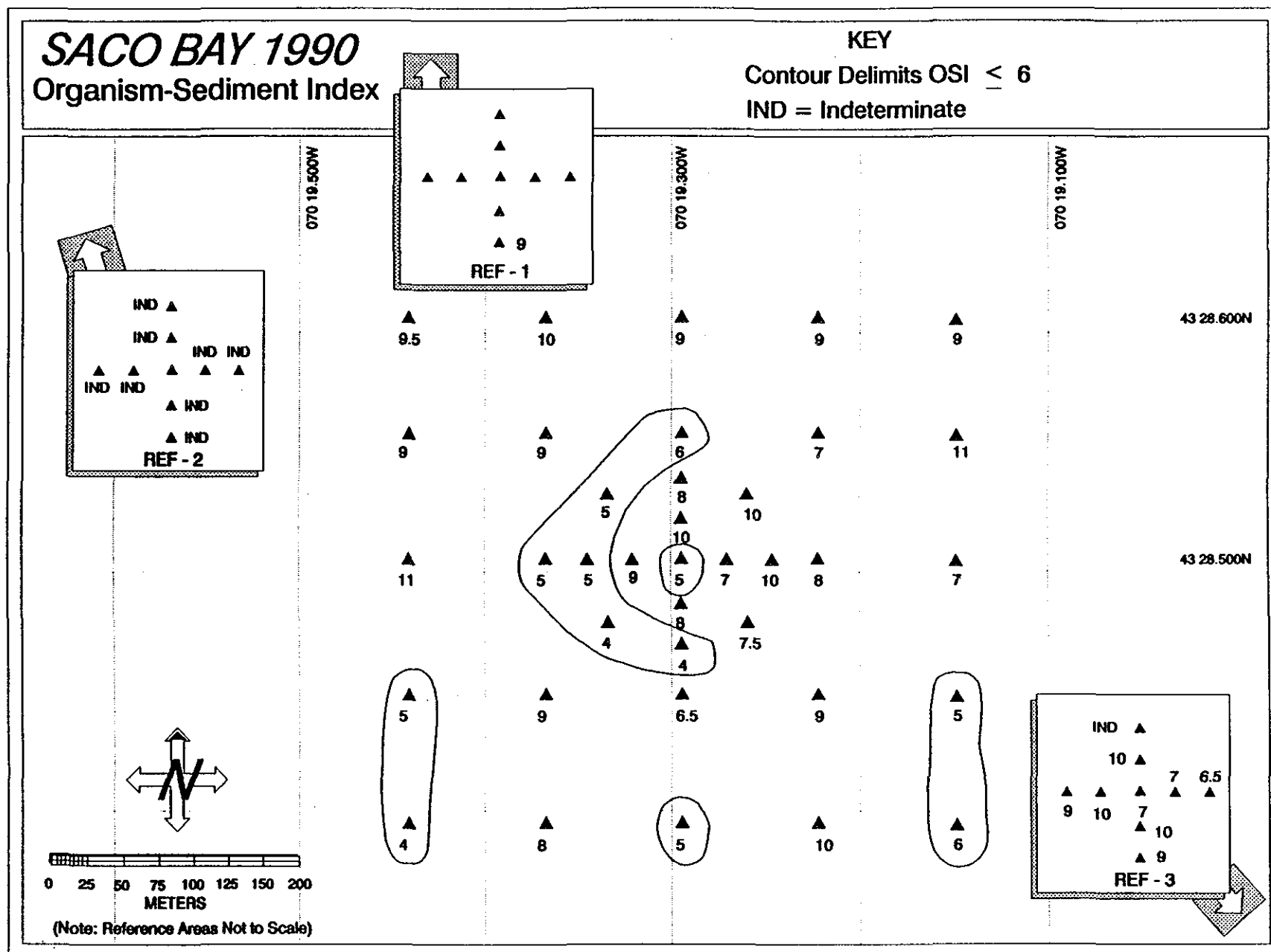
Figure 3-12. Mapped distribution of median Organism-Sediment Index (OSI) values at Saco Bay Disposal Site and reference stations, May 1990.
