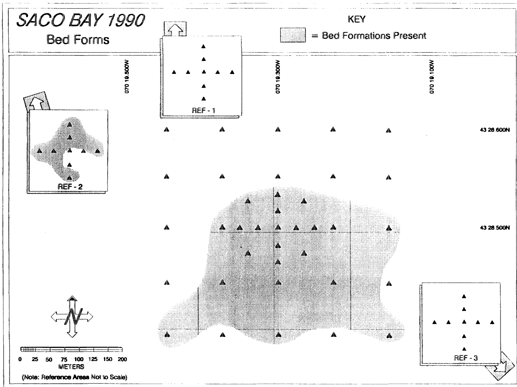
Figure 3-7. Mapped distribution of bed formations at Saco Bay Disposal Site and reference stations, May 1990.
