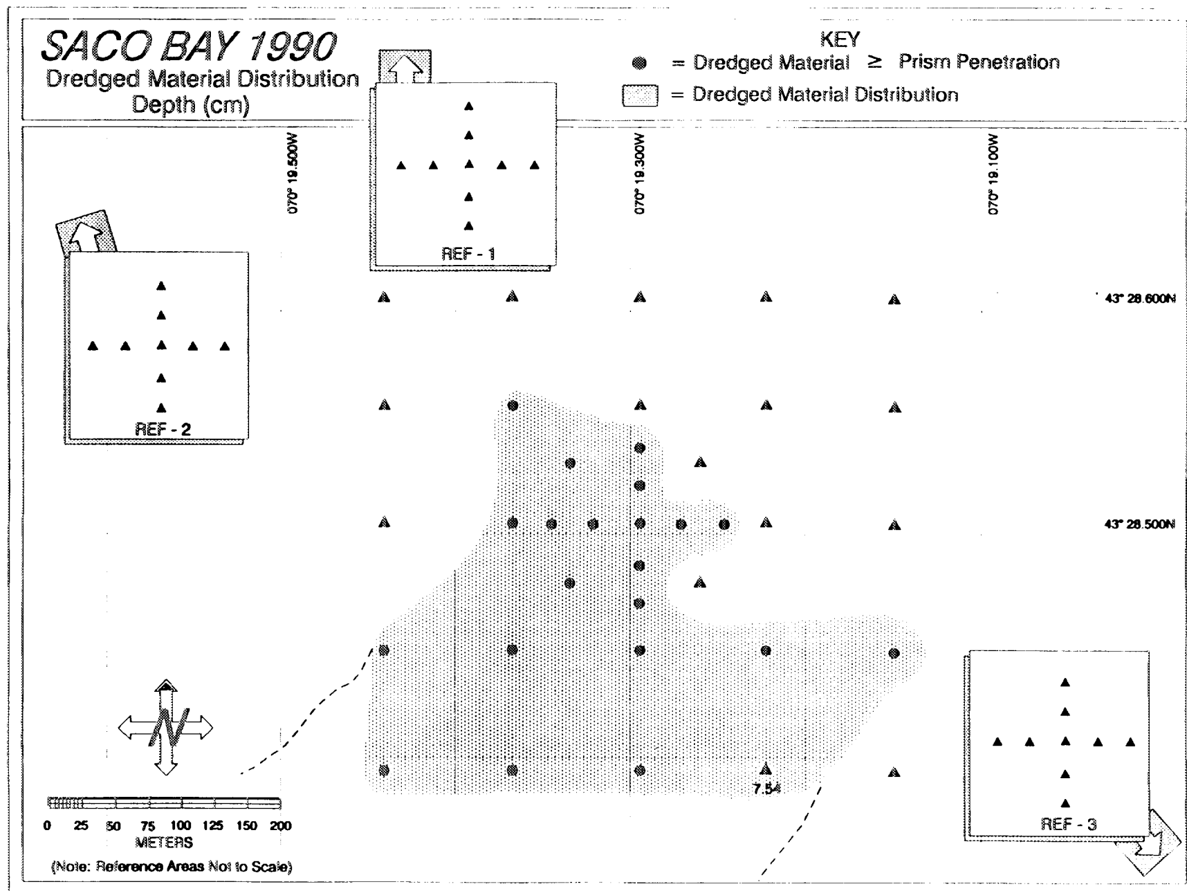
Figure 3-3. Distribution of dredged material based on REMOTS® photographs taken at Saco Bay Disposal Site, May 1990. Dotted line indicates possible extension of dredged material outside REMOTS® survey.
