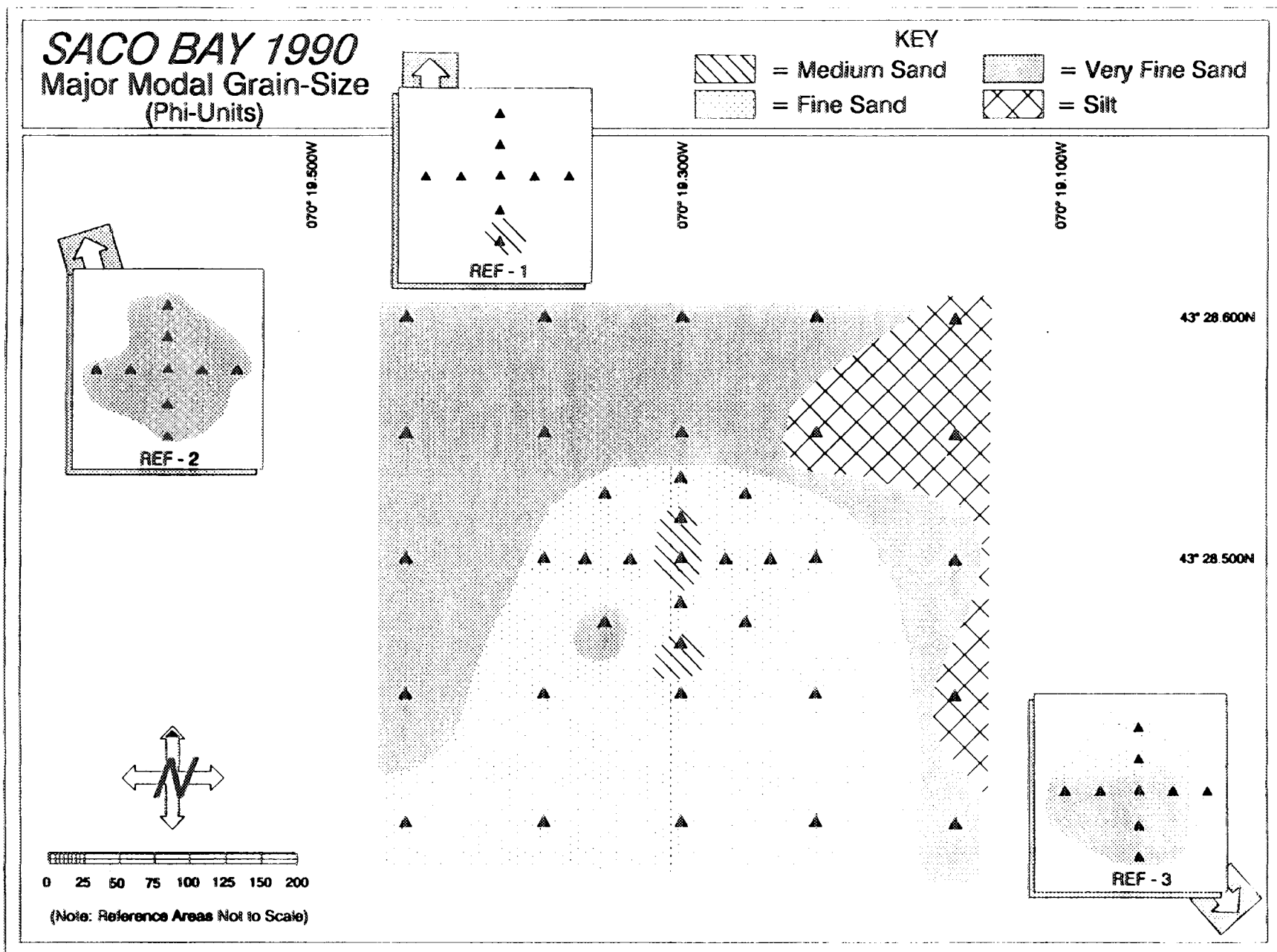
Figure 3-6. Mapped distribution of grain size major mode at Saco Bay Disposal Site and reference stations, May 1990.
