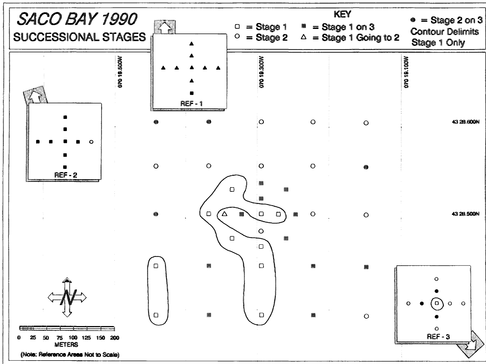
Figure 3-10. Mapped distribution of infaunal successional seres at Saco Bay Disposal Site and reference stations, May 1990.
