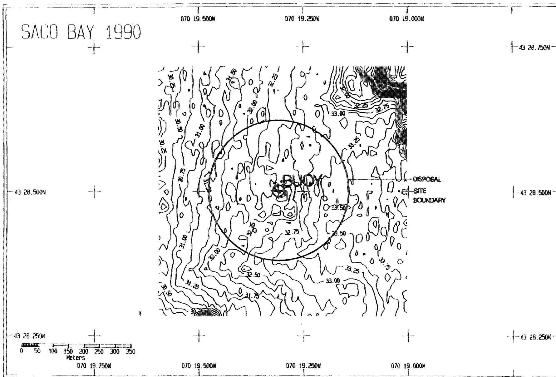
Figure 3-1. Bathymetric contour chart (800 X 800 m) of Saco Bay Disposal Site, May 1990.
