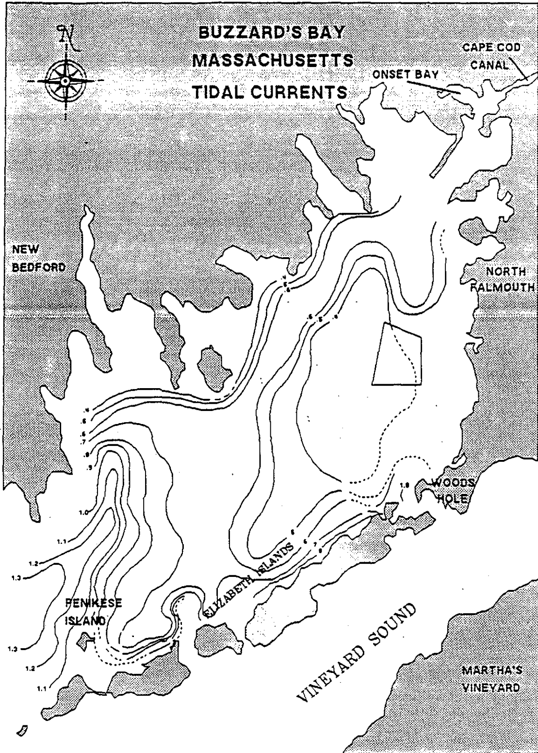
Figure 6. Tidal currents in Buzzards Bay (from Moore, 1963).
