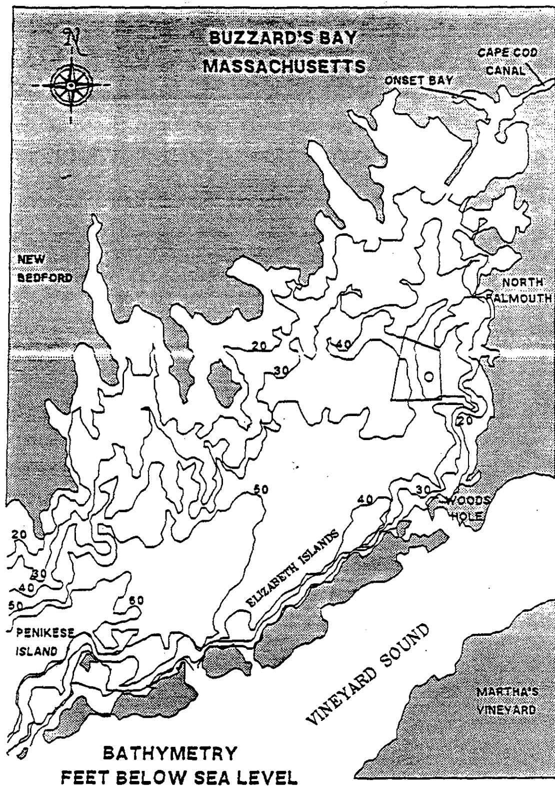
Figure 3. Buzzards Bay bathymetry chart (from Moore, 1963):
