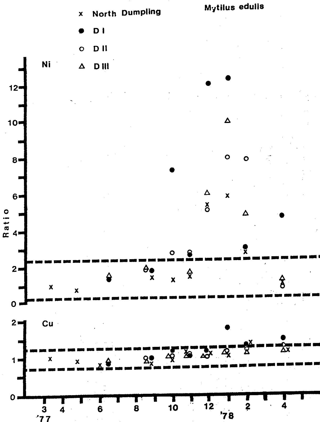
Figure 10. Temporal variation in the ratios of heavy metals in Mytilus edulis from New London monitoring sites: D I, D II and D III, as well as North Dumping, a reference site. Broken lines represent the 95% confidence limits of the baseline data.
