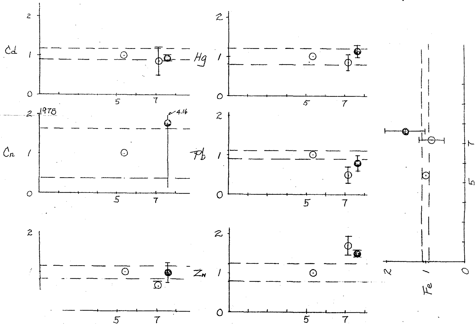
Figure E-4A Temporal variation in the ratios of heavy metals in Mytilus edulis from Newport Outer Bridge (O) deployed at Brenton Reef disposal site (●). Broken lines represent the 95% confidence limits of the baseline data.
