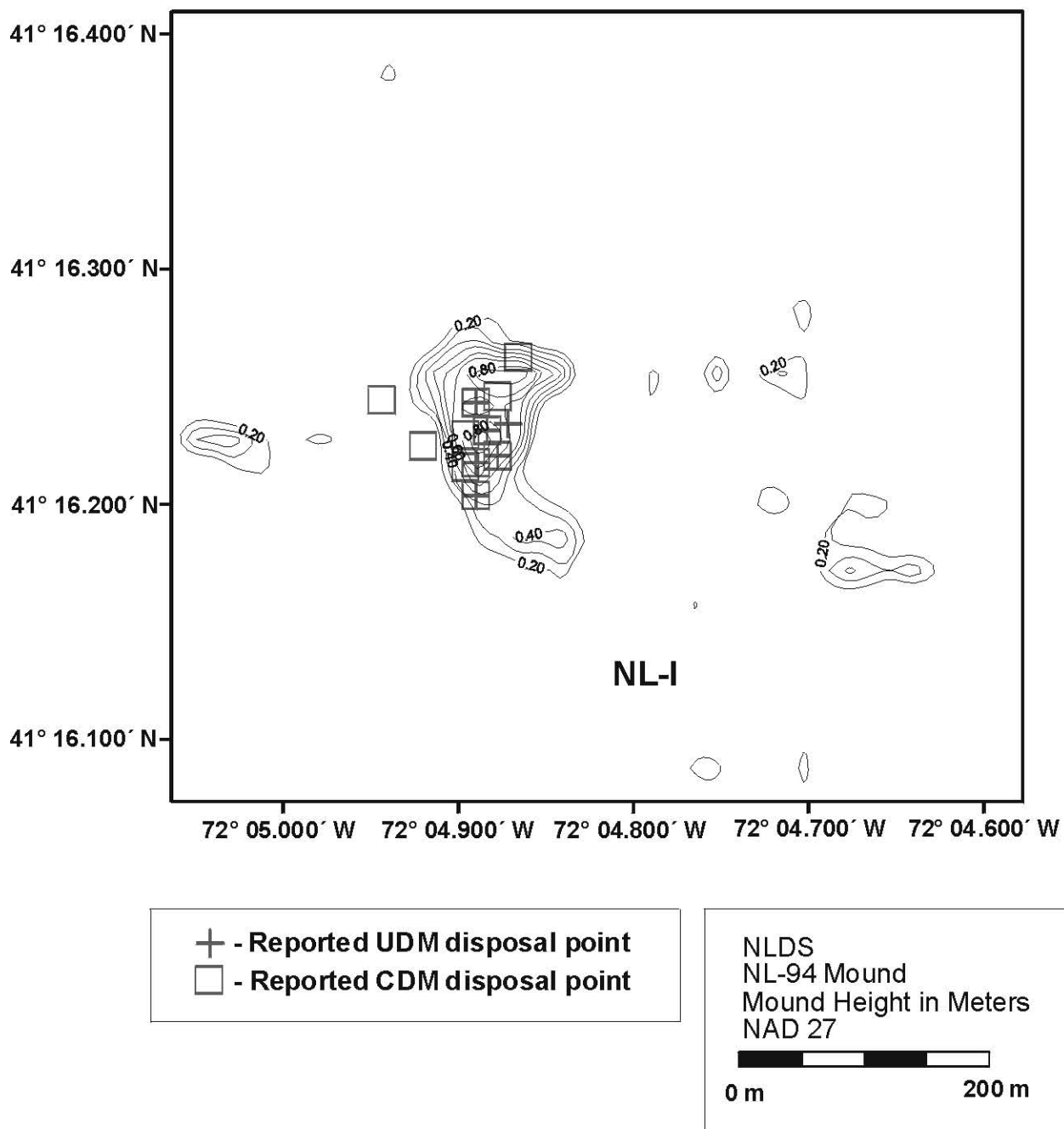
Figure 4-3. Reported barge disposal and capping positions over the NL-94 mound
