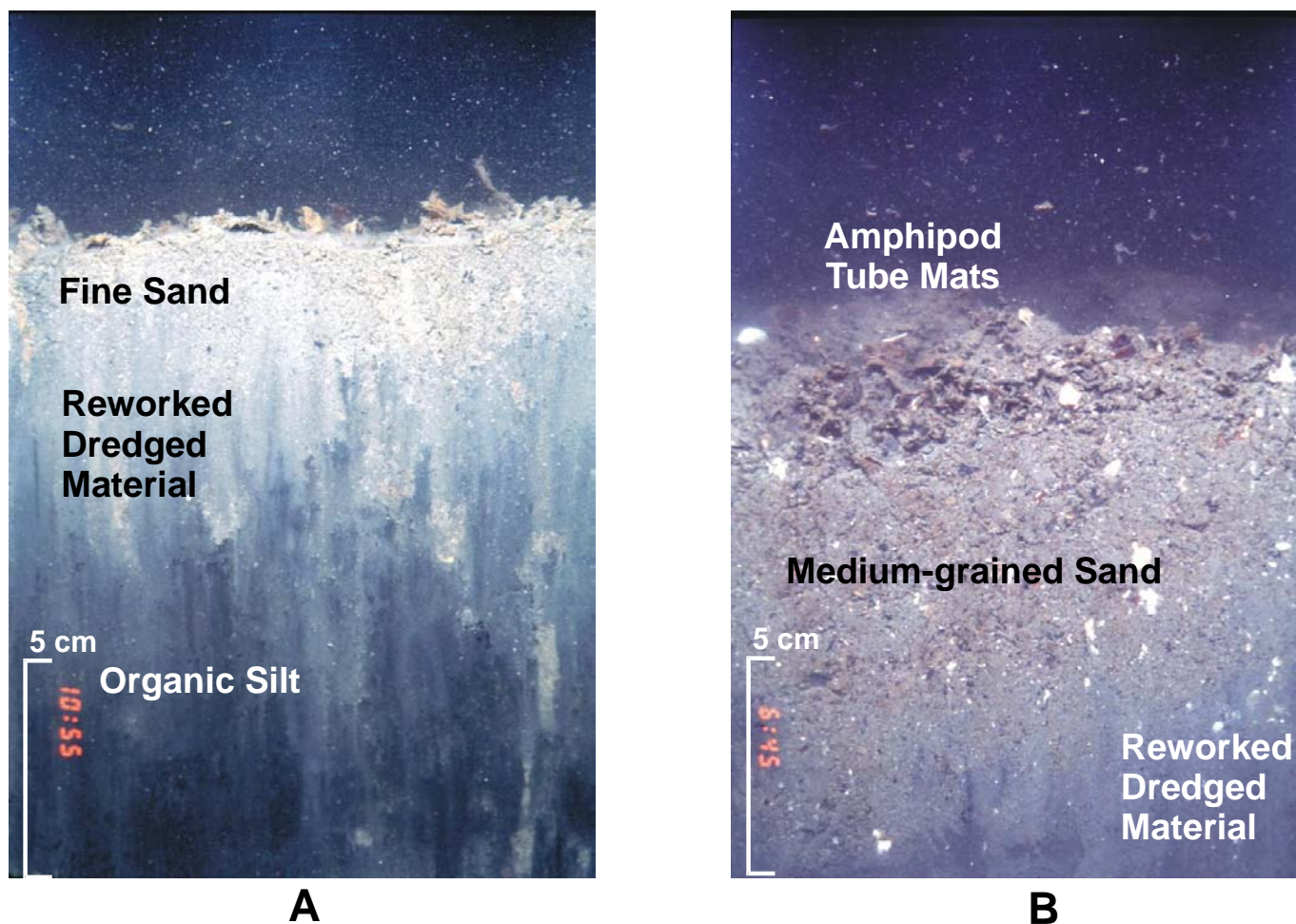
Figure 3-25. 1997 REMOTS® images from Stations 200E (A) and 200W (B) depicting dredged material layering and medium-grained sand in the surface layer, respectively
