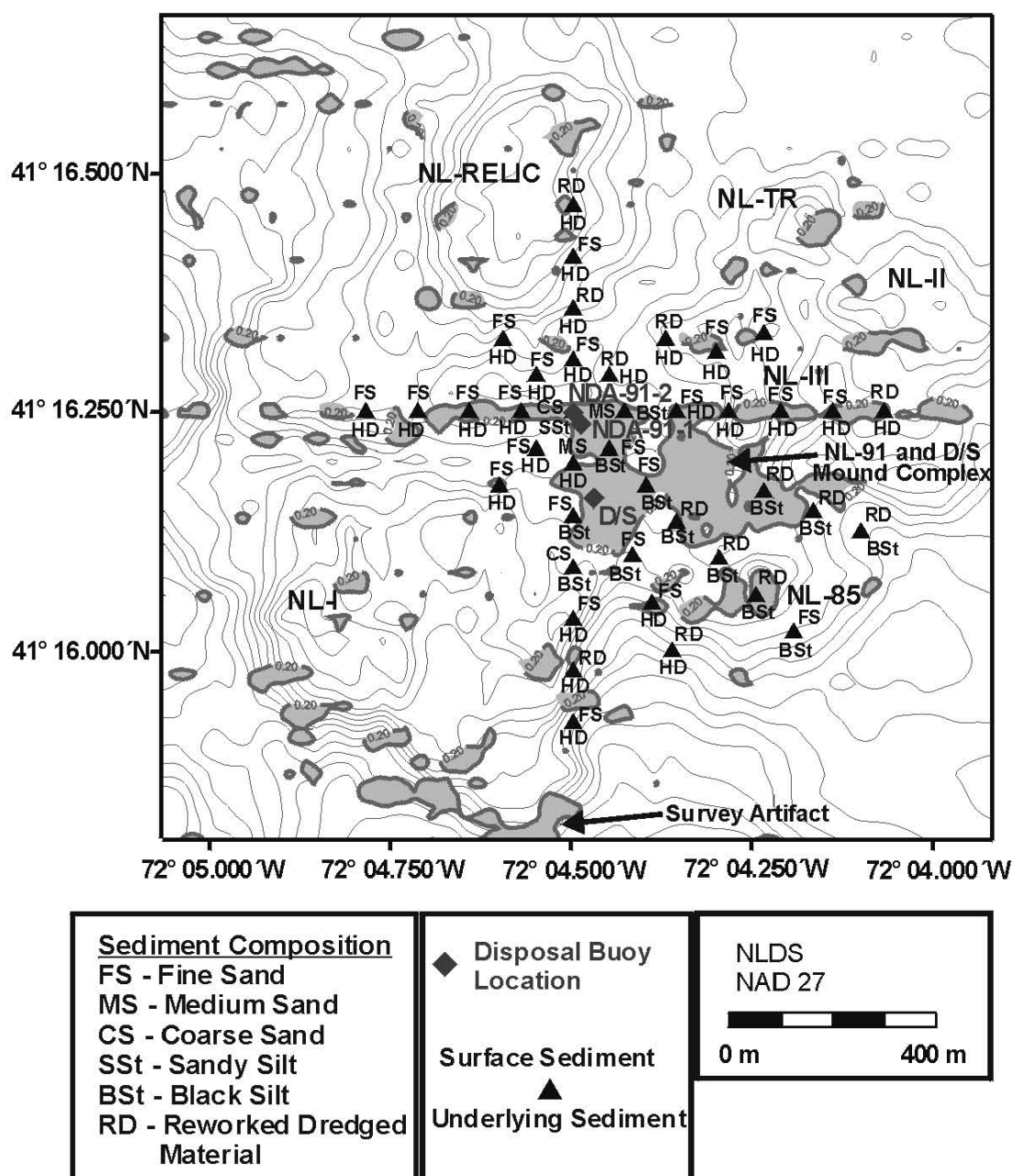
Figure 3-10. Distribution map of surface sediment type over fresh and/or historic dredged material in the vicinity of the new NL-91 and D/S mound complex at NLDS
