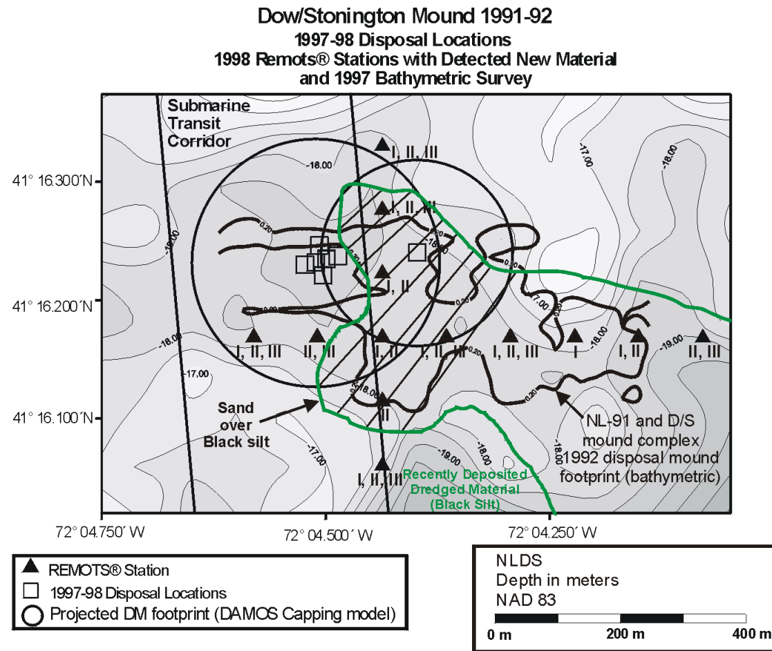
Figure 3-33. Distribution map of successional stage calculated for the 1998 survey over the NL-91 and D/S mound complex, relative to the 1992 disposal mound footprint and the predicted footprint of new material deposited during the 1997-98 disposal season
