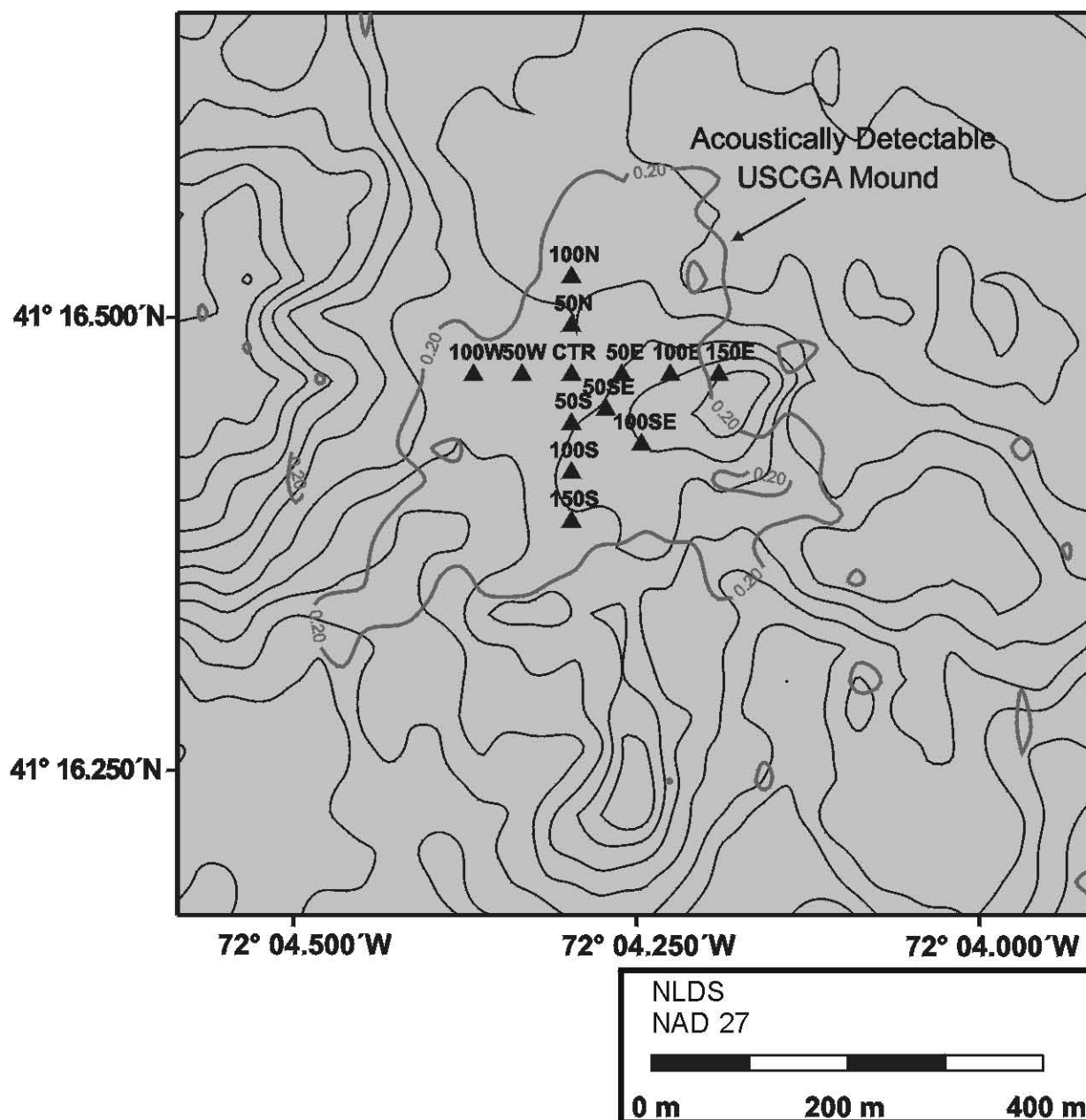
Figure 2-5. Distribution of 1995 REMOTS® sediment-profile photography stations (13) over the USCGA mound, relative to the detectable margins of the mound
