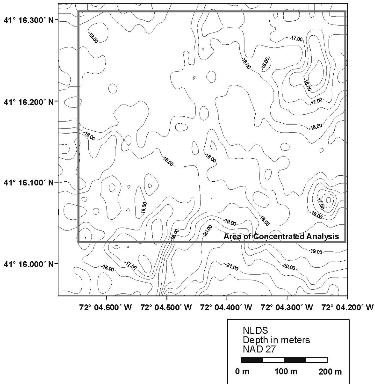
Figure 3-3. Bathymetric contour plot of the 940 m × 840 m survey conducted at the New London Disposal Site by Ocean Surveys Inc., in December 1991, 0.5 m contour interval
