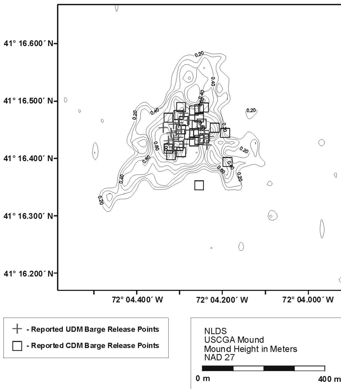
Figure 4-1. Reported barge release points, for disposal and capping, over the USCGA mound
