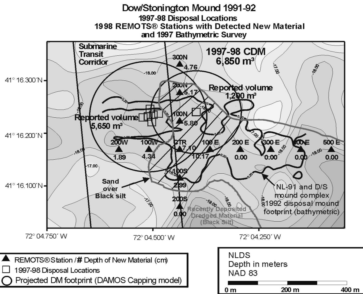
Figure 3-30. CDM disposal locations and projected footprint of new dredged material on the seafloor vs. depth of new material at REMOTS® stations over the NL-91 and D/S mound complex
