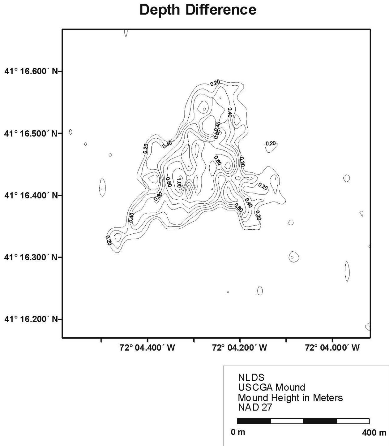
Figure 3-36. USCGA mound, depth difference from August 1992 to August 1995, 0.2 m contour interval
