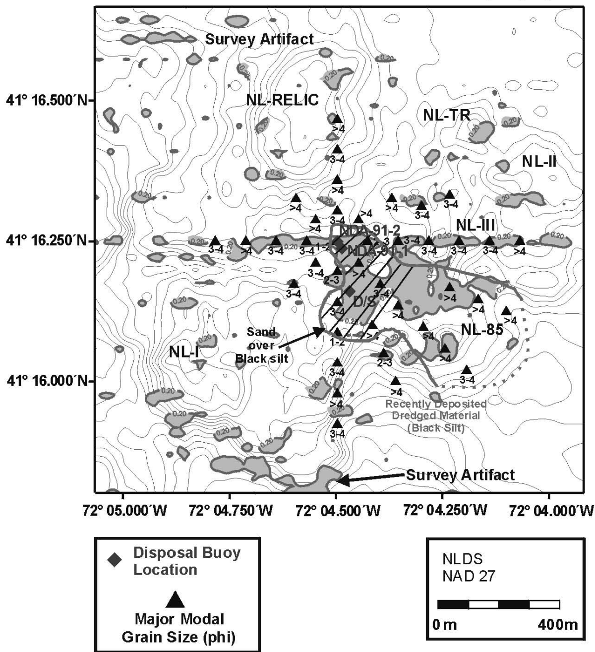
Figure 3-14. Spatial distribution of the major modal grain size for the 1992 REMOTS® sediment-profile photography stations over the NL-91 and D/S mound complex
