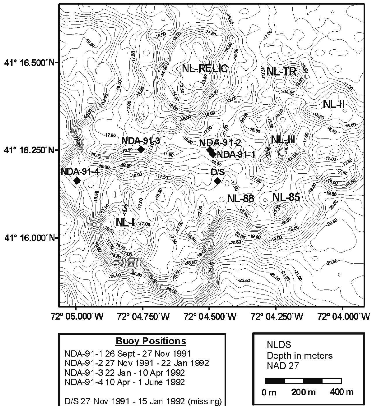
Figure 3-1. Bathymetric contour plot of the 1600 m × 1600 m survey area over the New London Disposal Site, August 1992. A 0.25 m contour interval shows current and relic disposal mounds
