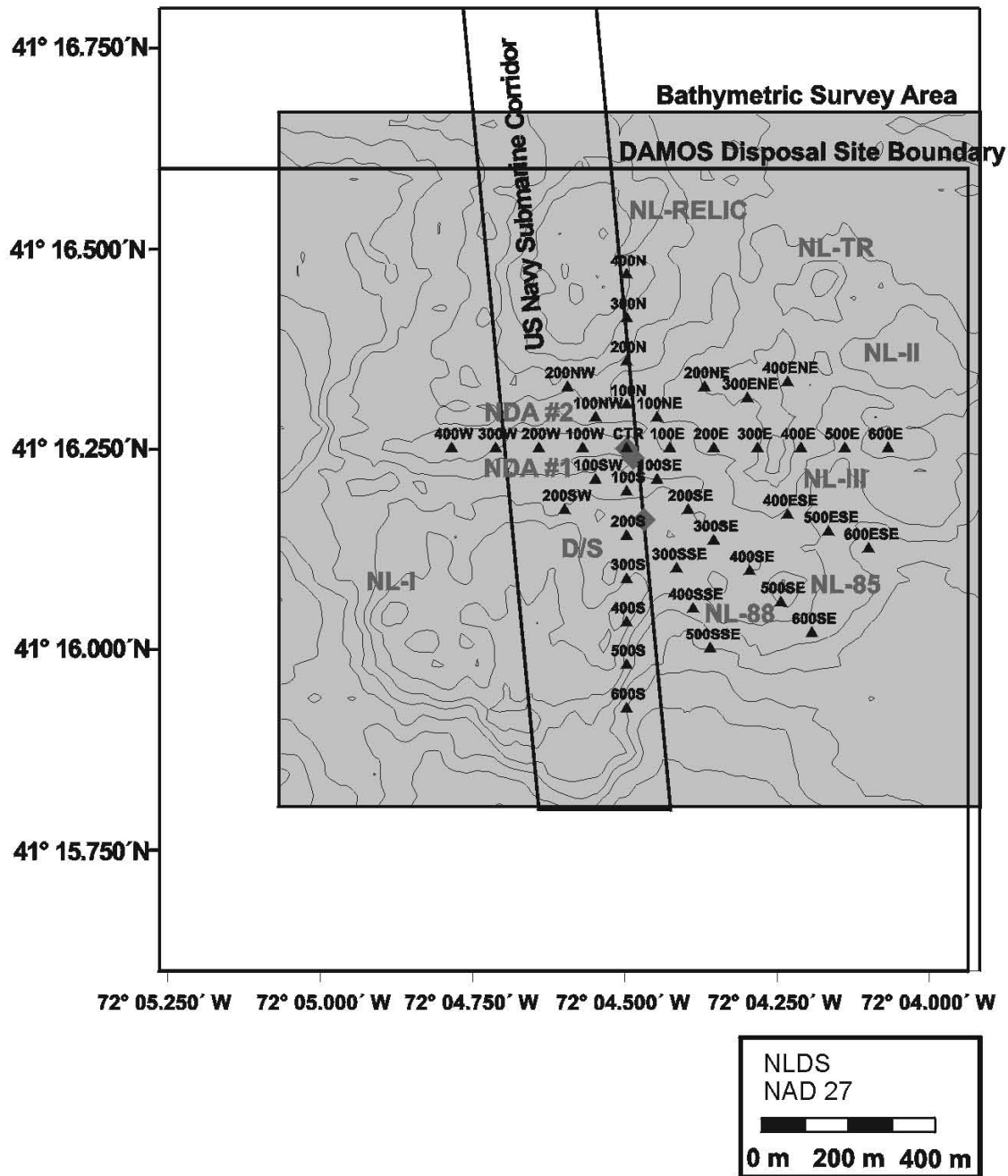
Figure 2-4A. Distribution of the 1992 REMOTS® sediment-profile photography stations (41) over the NL-91 and D/S mound complex, relative to the DAMOS disposal site boundary and the U.S. Navy submarine corridor
