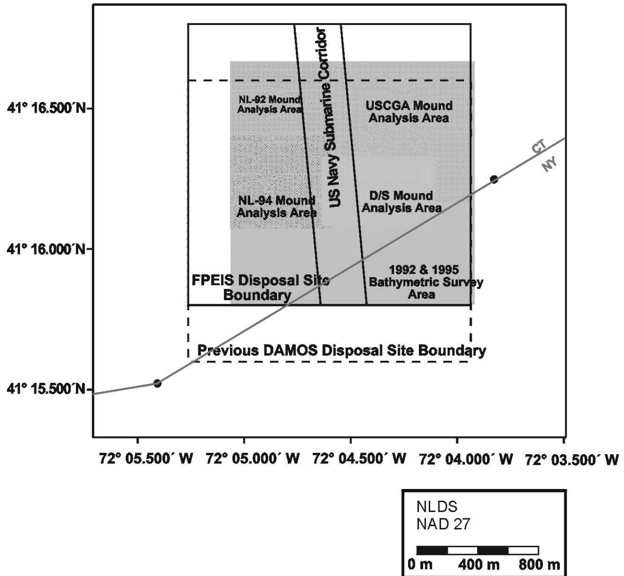
Figure 2-1. Location of the 1992 and 1995 bathymetric survey area over NLDS, relative to the disposal site boundaries, analysis areas for individual mounds, and the New York and Connecticut State Line (NAD 27)
