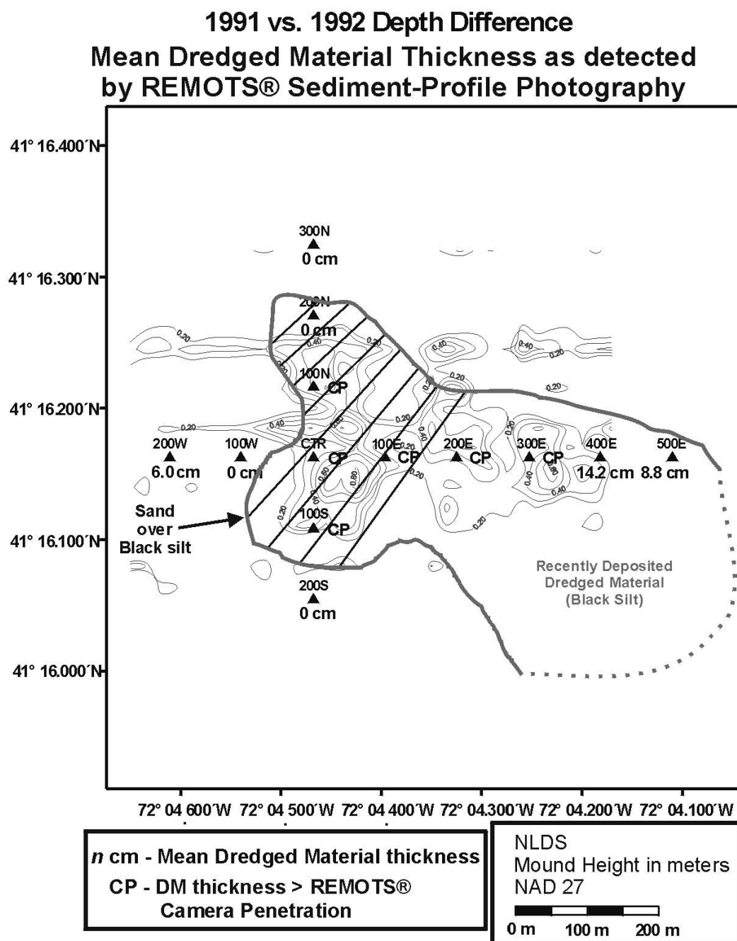
Figure 3-20. Mean dredged material thickness at 1995 REMOTS® sediment-profile photography stations over the NL-91 and D/S mound complex, relative to the August 1992 detectable margins
