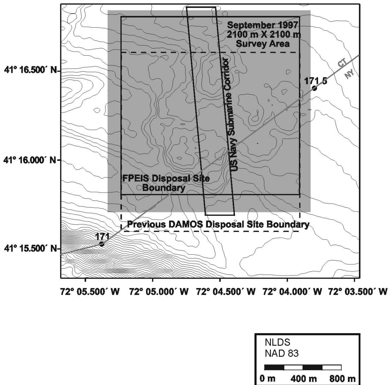
Figure 2-2. Location of the 1997 master bathymetric survey area over NLDS, relative to the disposal site boundaries and the New York and Connecticut State Line (NAD 83)
