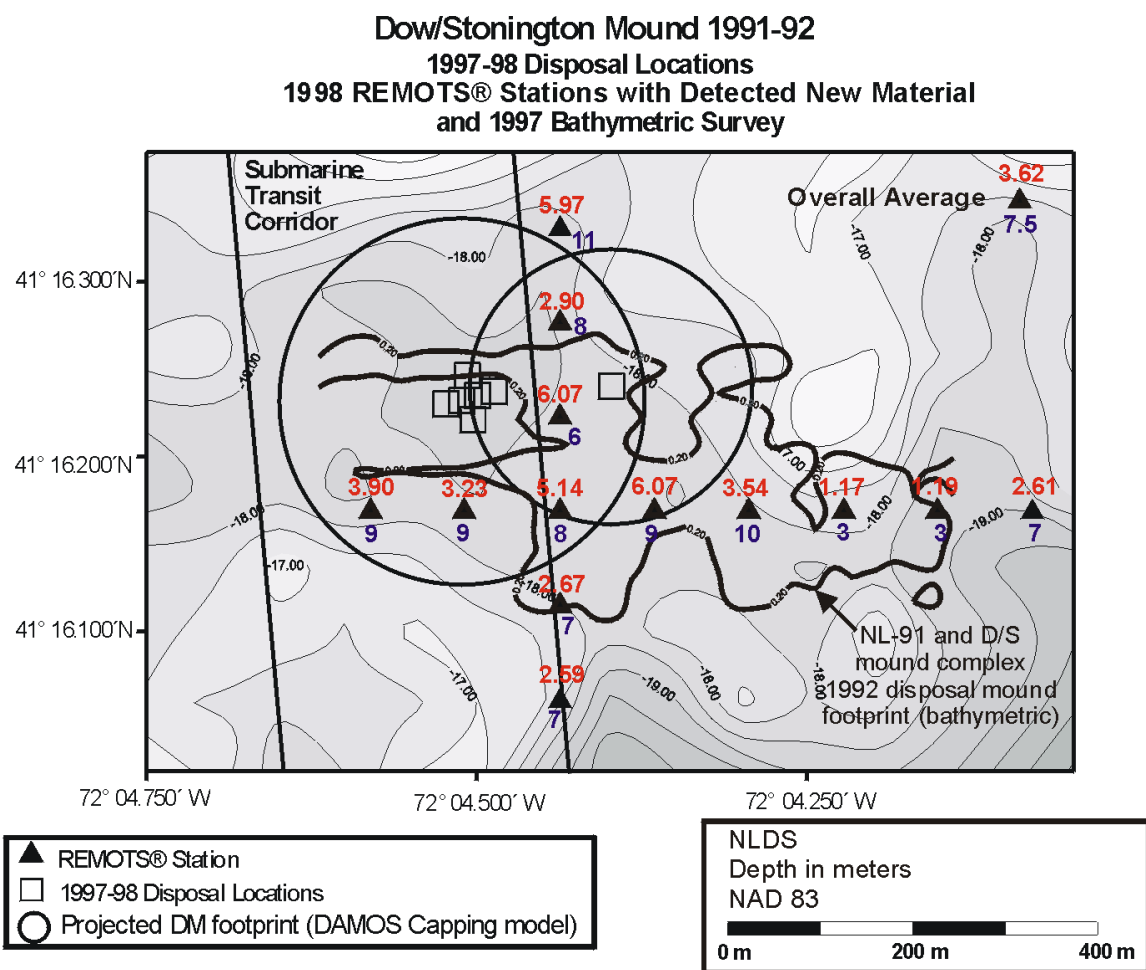
Figure 3-32. Distribution map of mean RPD (red) and median OSI (blue) values calculated for the 1998 survey over the NL-91 and D/S mound complex, relative to the 1992 disposal mound footprint and the predicted footprint of new material deposited during the 1997-98 disposal season
