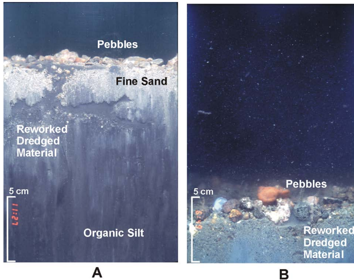
Figure 3-26. 1997 REMOTS® images collected at the NL-91 and D/S mound complex Stations 100S (A) and 200S (B) displaying a surface layer of pebbles over reworked dredged material
