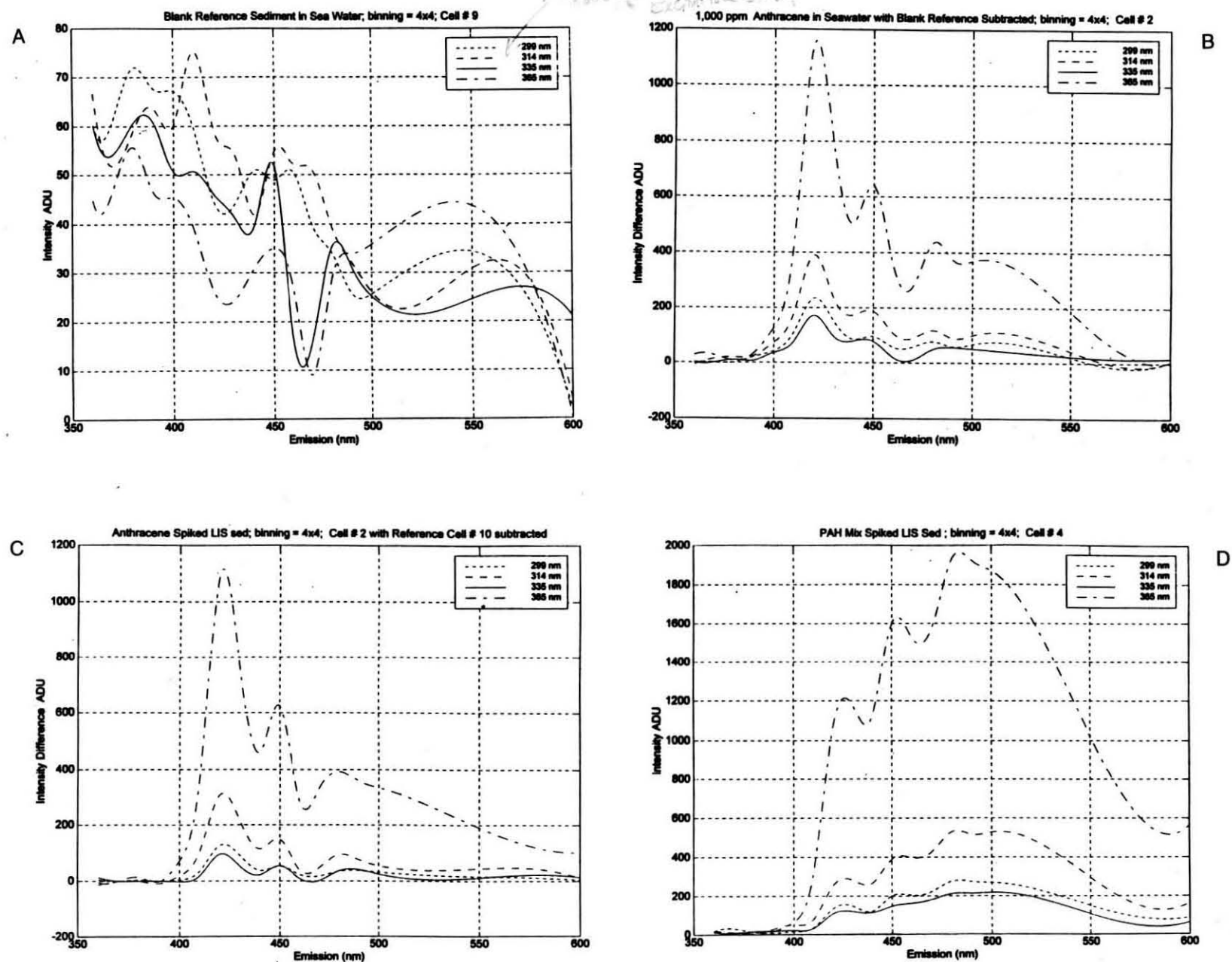
Figure 2. Results of UV-REMOTS laboratory analysis of anthracene (ANT) spiked water and sediments: A) Reference sediment in seawater; B) ANT and seawater; C) ANT and sediment; and D) Sediment PAH mix with ANT.
