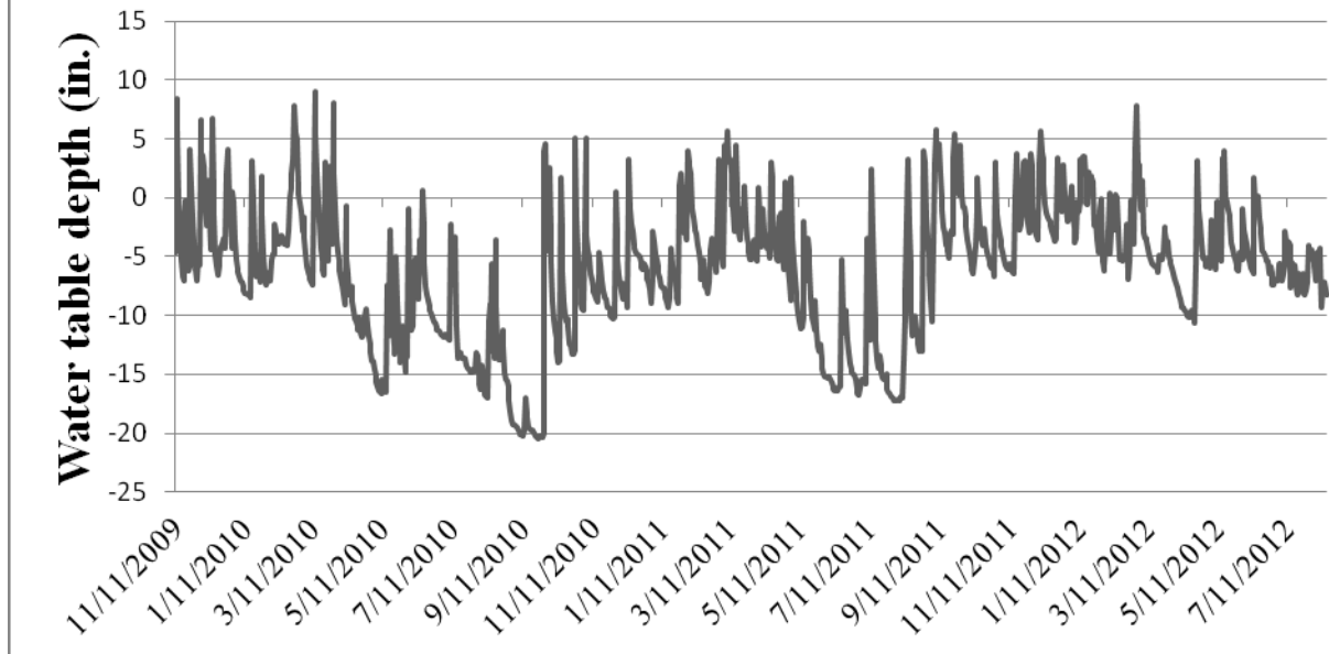
Fig. 11. CHb Hydroperiod
