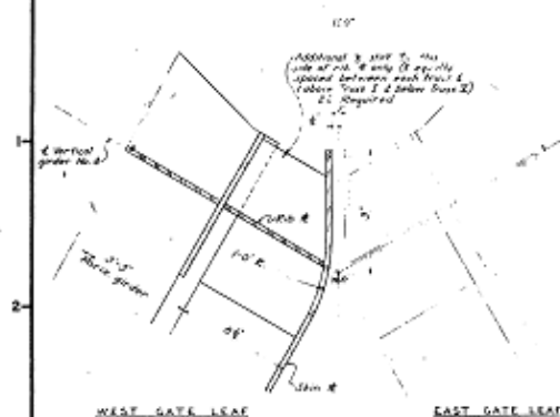
PLAN CLOSURE DETAILS SCALE 1/4" = 1'-0"
