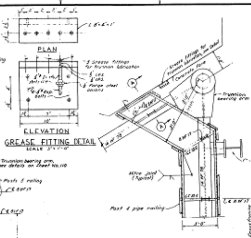
PART PLAN
