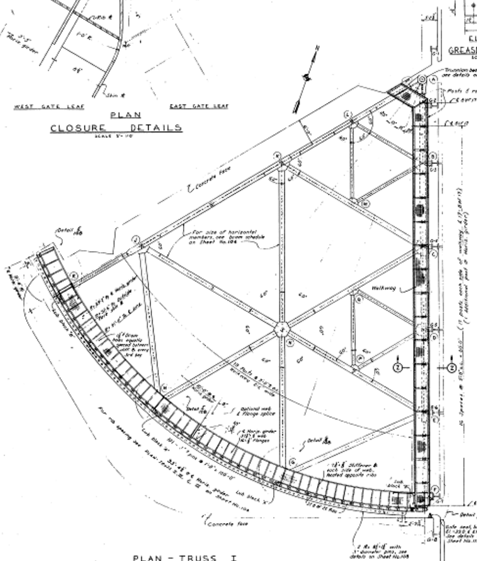
PLAN - TRUSS I
