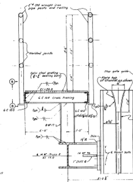
SECTION Z-Z
