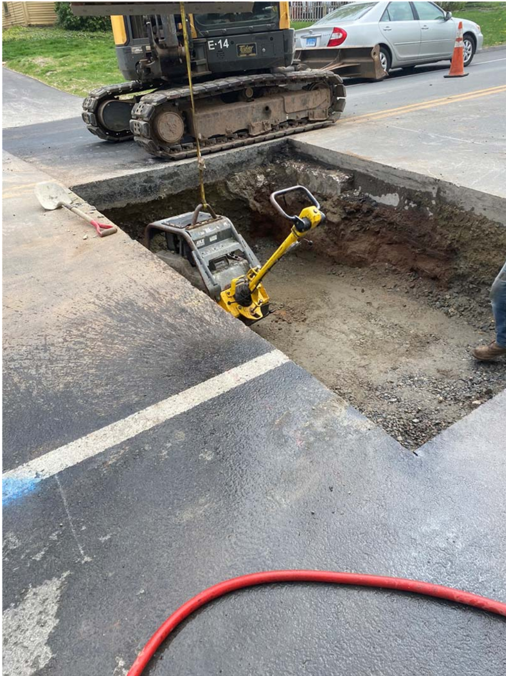
Picture 2: Ludlow begins to backfill and compact the trench in 6" lifts. Trench is compaction tested after each lift by John Turner Testing. All results are between 95-98%. View to the north.
