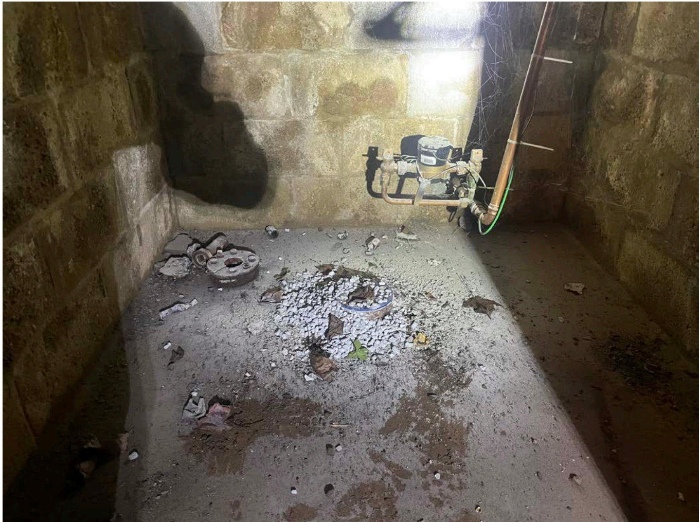
Picture 3: The well located in the basement of the 127 Main Street, Durham, residence on the west side of the foundation after Grela filled the well with bentonite chips and placed an expansion plug on the steel casing as part of well decommissioning activities. View to the west.
