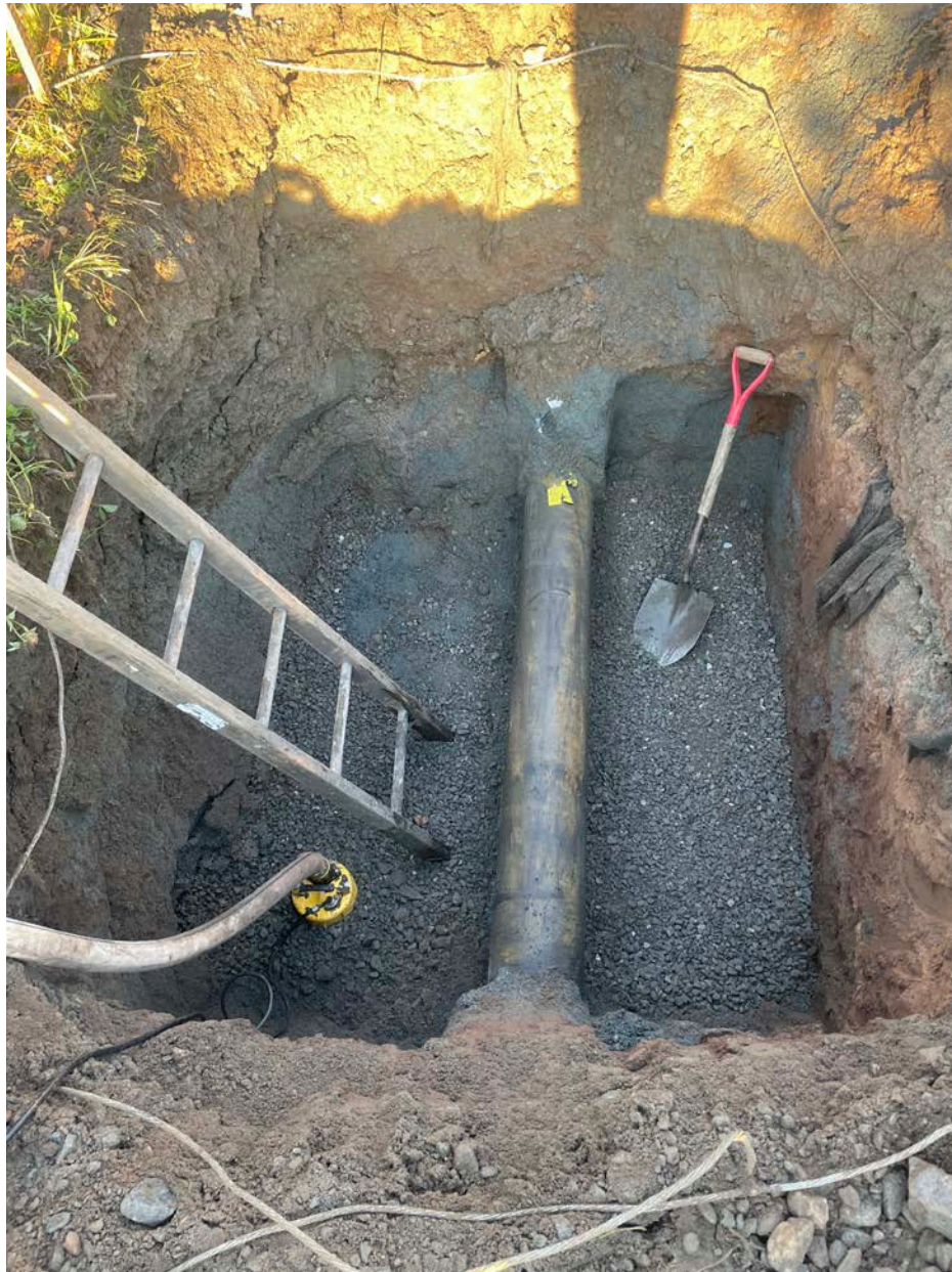
Picture 2: Section of 8" DIP that Ludlow daylighted on the north side of the Booster Station as they work to install an 8" DIP gate valve. View to the west.
