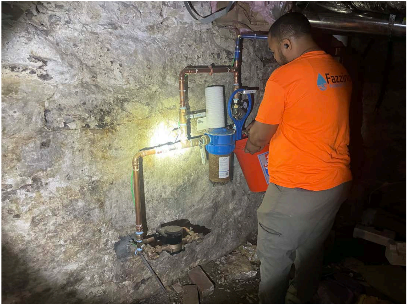
Picture 14: Fazzino Plumbing changing the filter on the water system they previously installed at the 313 Main Street, Durham, residence.
