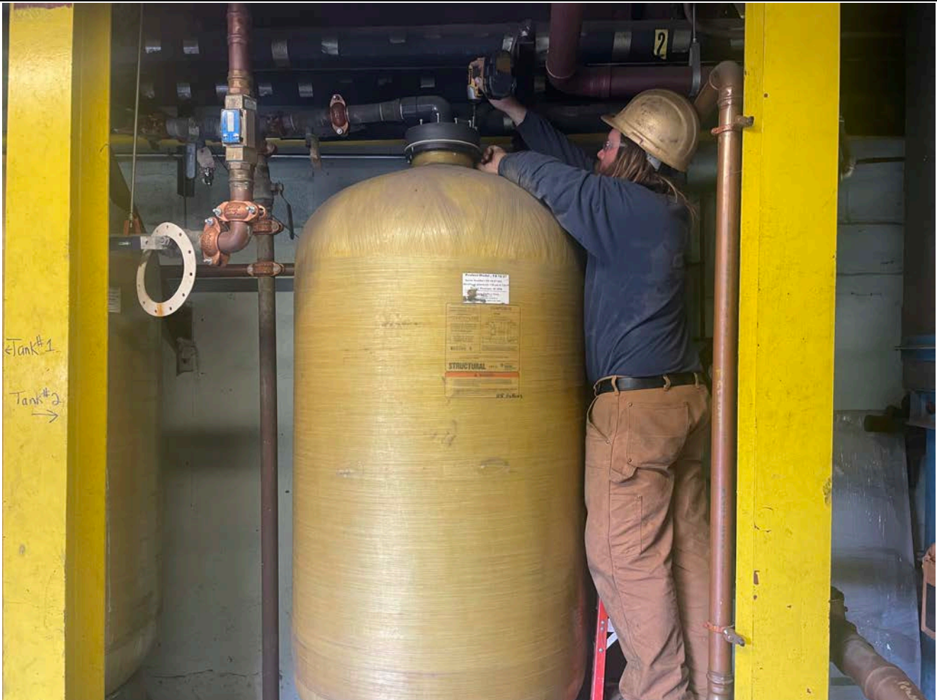
Picture 4: West State Mechanical removing the top from a GAC vessel in order to allow Farrar Filter Co. Inc. to remove the carbon located within. View to the south.
