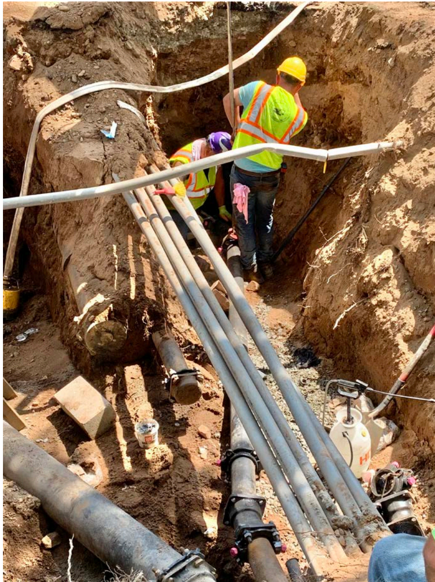
Photo 4: Ludlow Construction capping the former domestic water service at Korn School.
