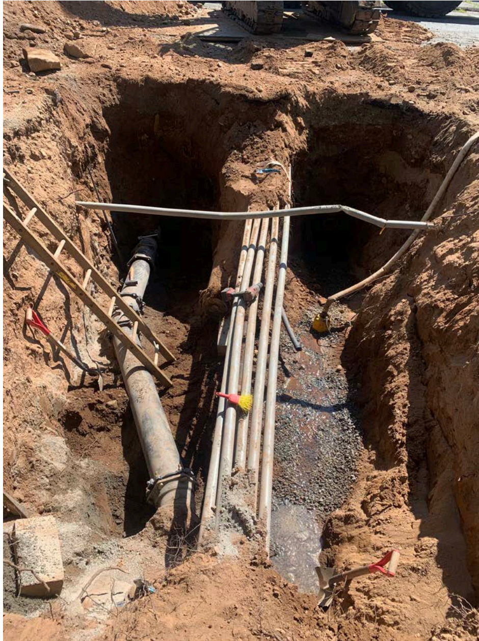
Photo 2: Ludlow Construction connecting the fire service at the former Korn School.
