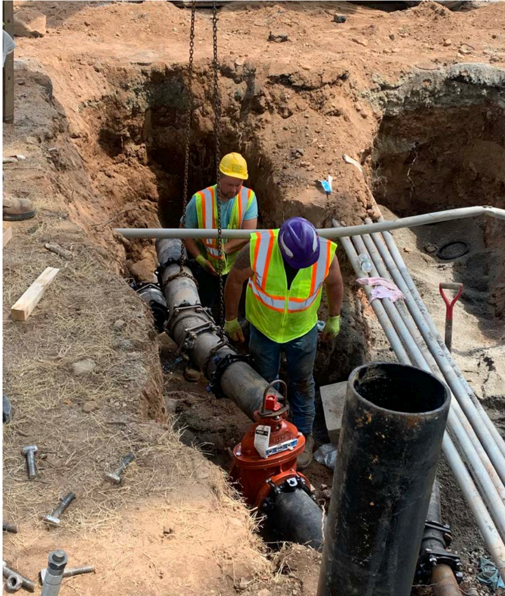
Photo 5: Ludlow Construction is working on tying in the 8-inch fire service.
