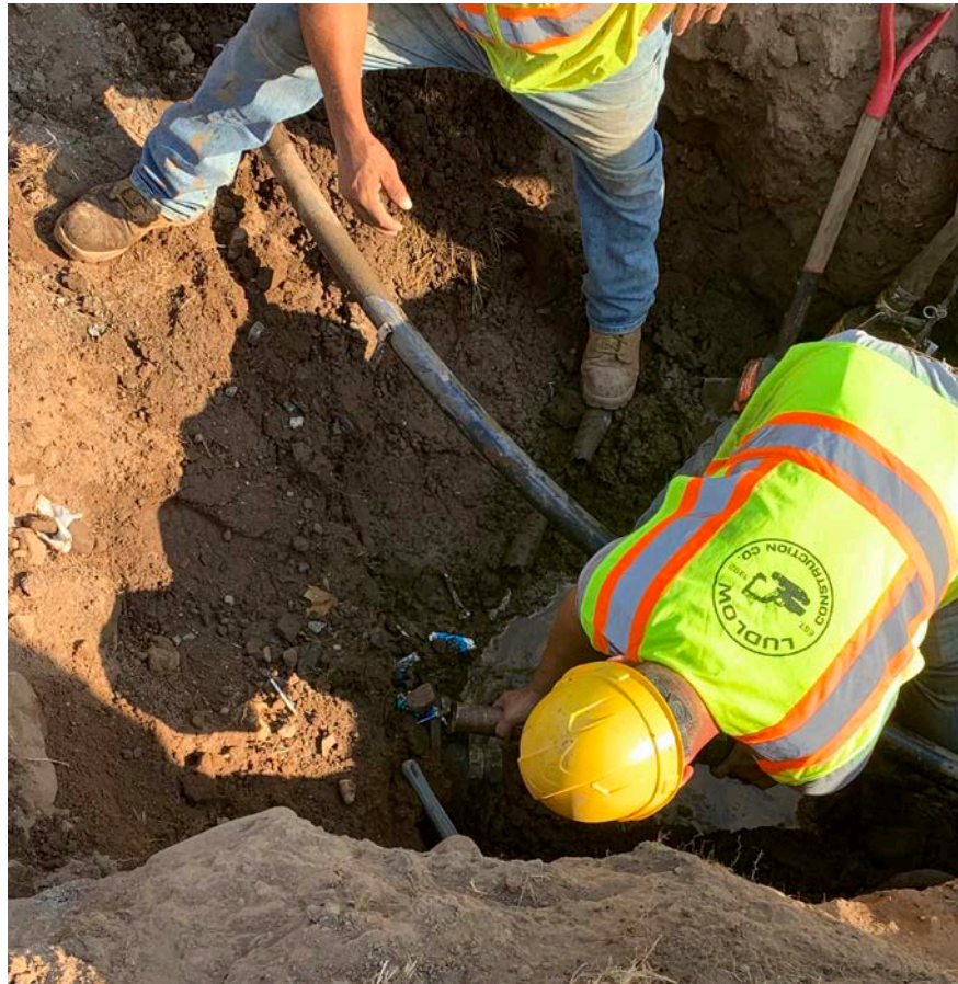
Picture 2: Ludlow Construction is tying in a newly installed pipe to the existing District 13 sprinkler system vault.
