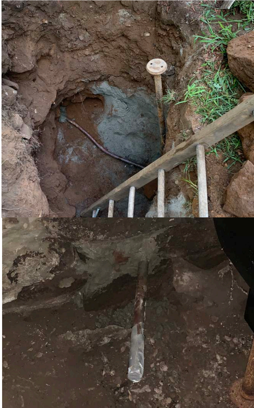
Picture 1: Ludlow Construction at 63 Maiden Lane installing a water service. (First image represent the outside side of the building foundation, the second image represents the inside side of the building foundation.)
