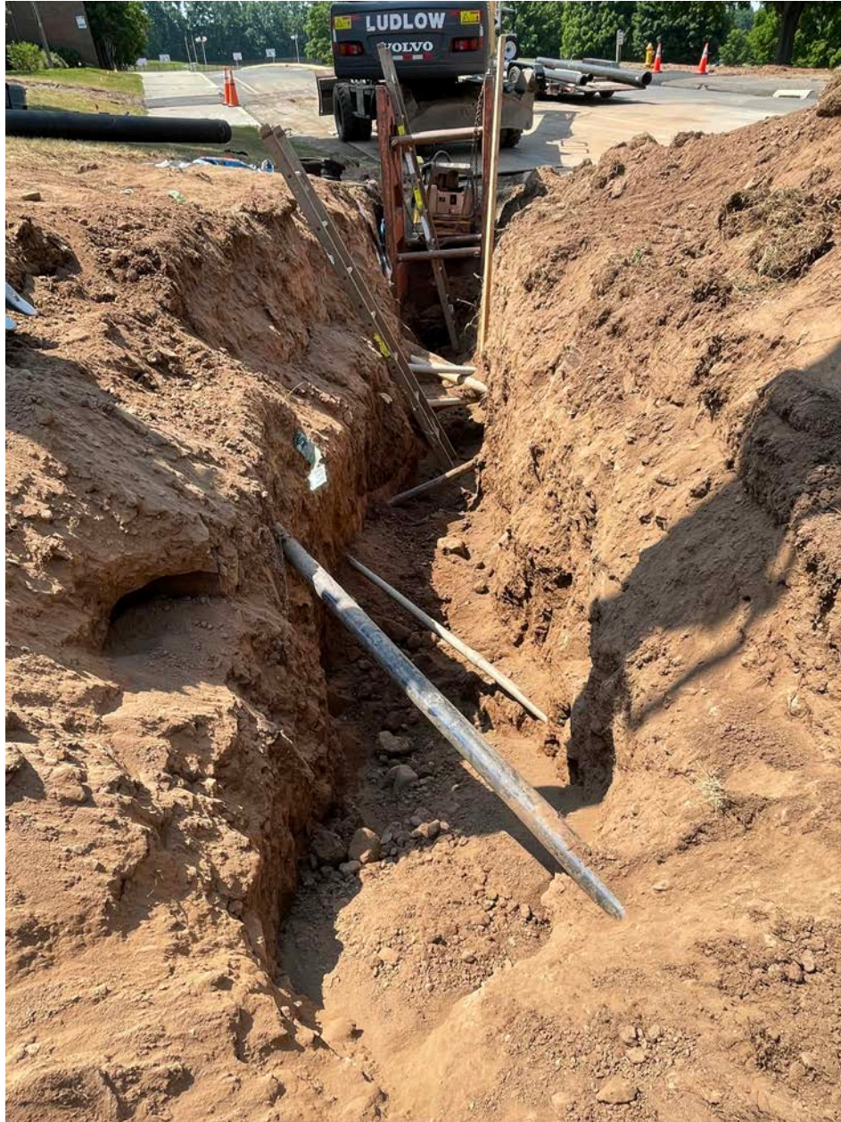
Picture 7: Some of the subsurface utilities that Ludlow daylighted today as part of installing 8" DIP approximately 30'-70' southwest of the water lien vaults at the CRHS property. View to the southwest.
