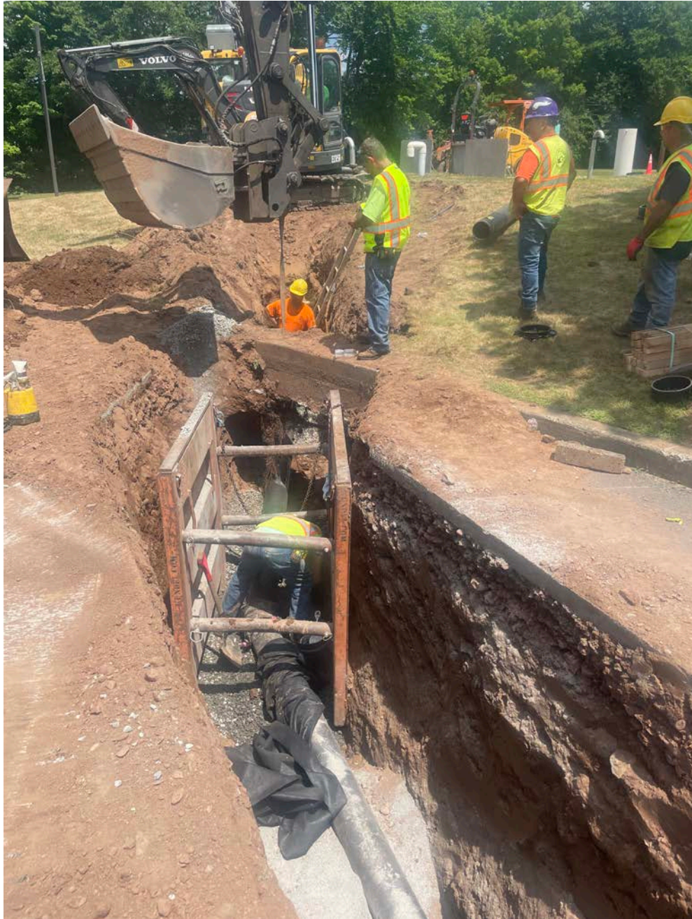
Picture 4: Ludlow connecting sections of 8" DIP together as they work towards the existing water line vaults located at the CRHS. View to the east.
