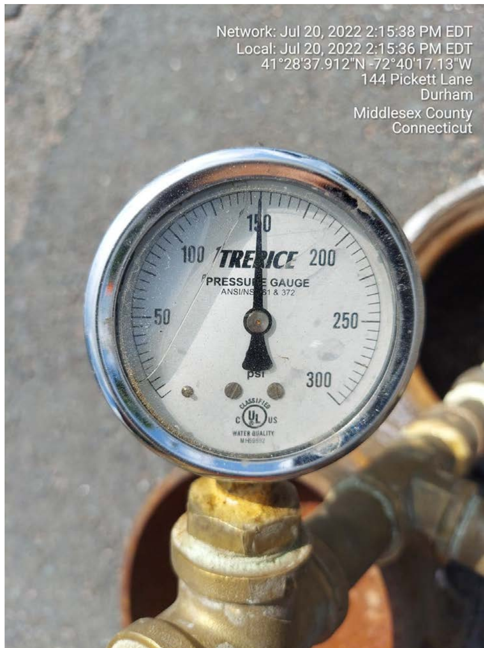
Picture 9: Starting pressure on the 4" DIP water line that Ludlow pressure tested today at Station 529+64.
