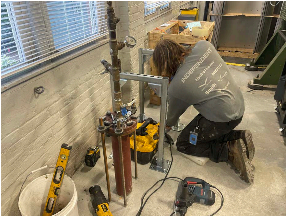
Picture 1: West State Mechanical securing the second section of the backflow preventer stand on the north side of the water service line that Ludlow previously brought into the Durham Manufacturing facility through the west side of the building. View to the northwest.
