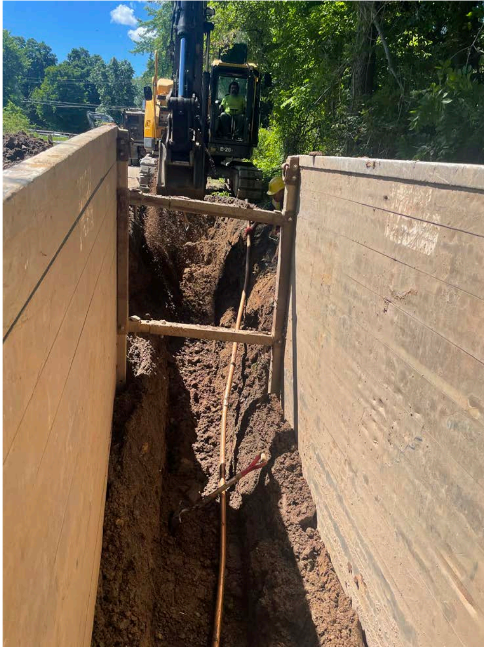
Picture 6: Ludlow installing 2" copper water service line on the south side of the Ball Brook culvert located on the 114 Maiden Lane driveway. View to the south.
