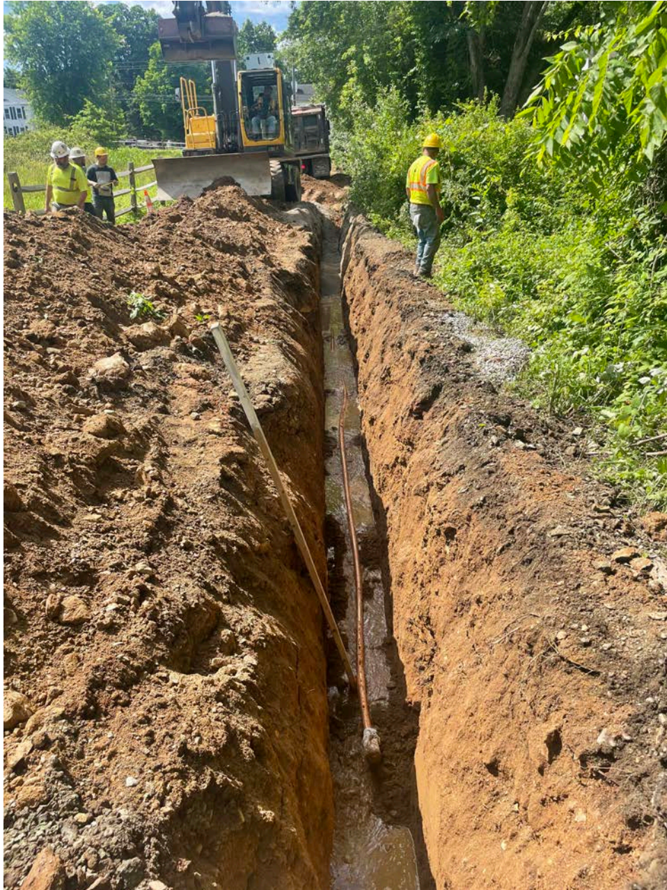
Picture 4: 2" copper water service line that Ludlow is in the process of installing on the west side of the 114 Maiden Lane, Durham, driveway. View to the south.
