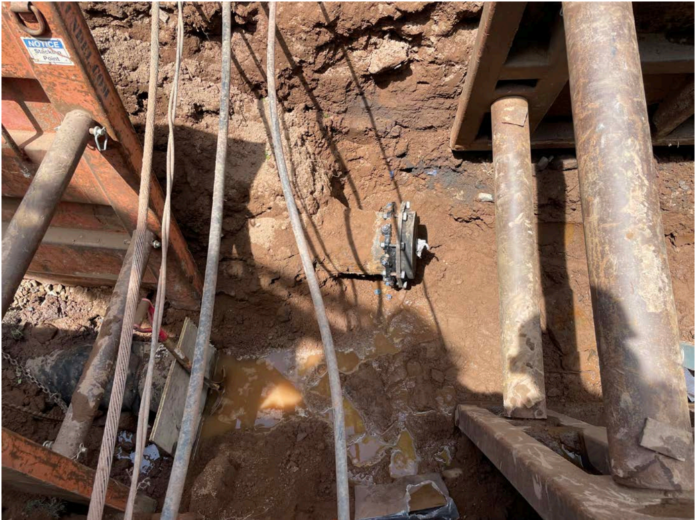
Picture 9: Section of 12" DIP that Ludlow placed a DIP plug onto at Station 40+41 on Talcott Ridge Drive in Middletown. View to the west.
