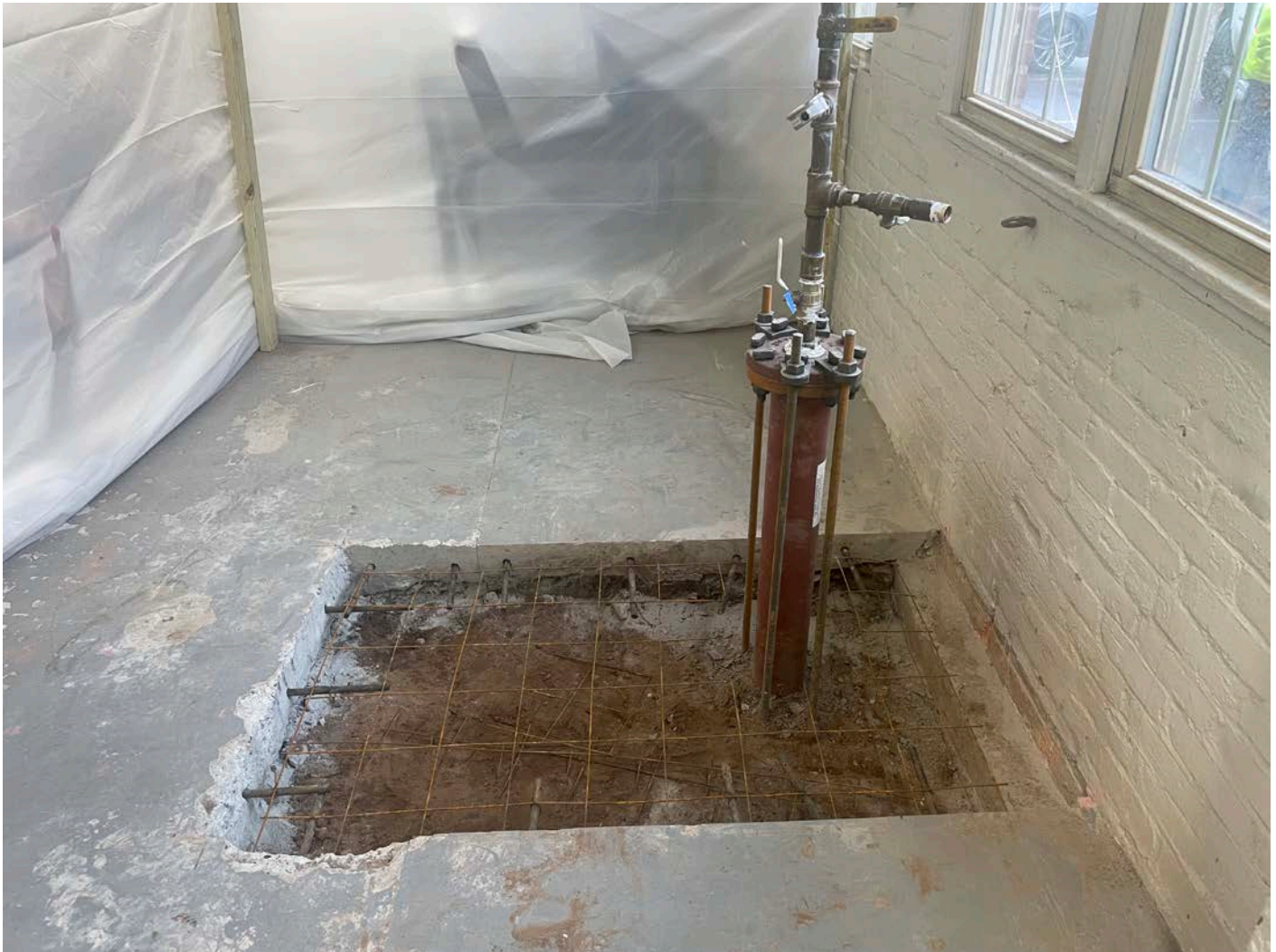
Picture 8: Hole in the floor of the Durham Manufacturing facility where Ludlow brought in a 4" DIP water service line. View to the south. Ludlow has placed steel screen and sections of rebar set into the sidewalls of the cut concrete as they prepare to fill the hole with concrete. View to the south.
