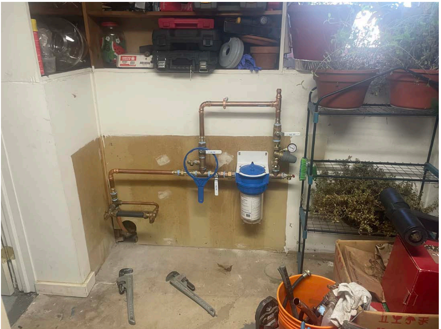
Picture 4: Partial installation of final water system components at the 230 Maple Avenue, Durham, residence by Fazzino Plumbing.
