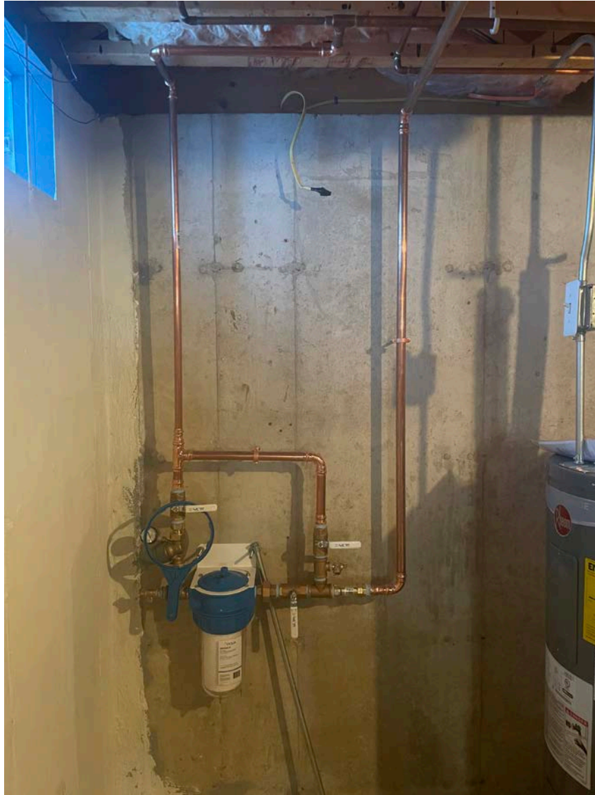
Picture 2: Final water system components that were installed at the 166 Maple Avenue, Durham, residence by Fazzino Plumbing.
