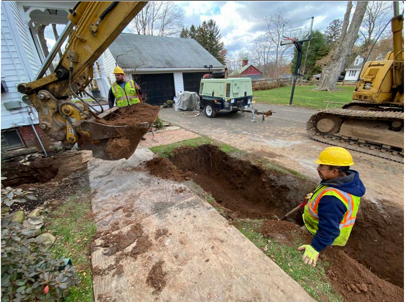
Picture 7: Ludlow backfills the trench of the 1" copper water service line to 254 Maple Ave residence with native fill. Looking west.
