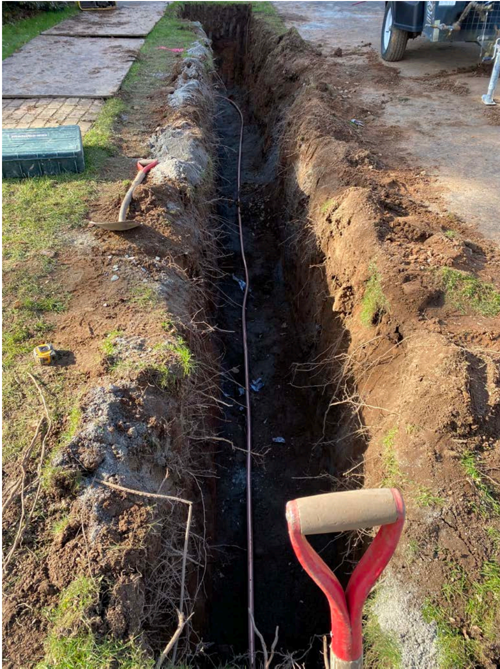
Picture 5: Ludlow places the 1" copper service line in the trench for the 254 Maple Ave residence. property in Durham. Looking west.
