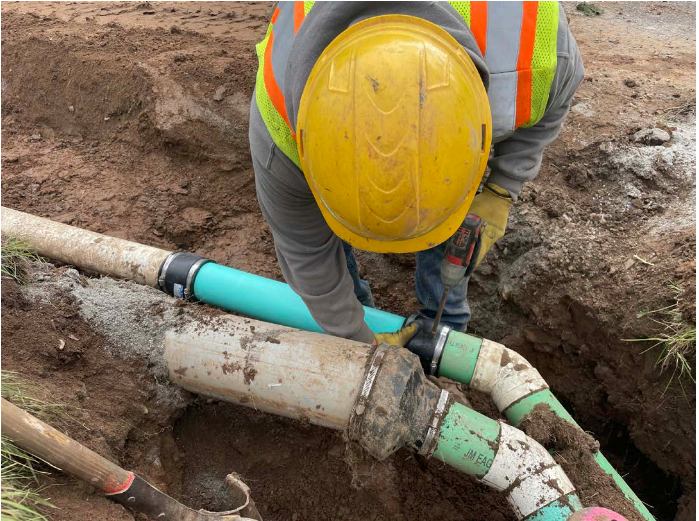
Picture 12: Ludlow repairing a 4" PVC drain line at the 173 Maple Avenue property with 4" PVC pipe and Fernco boots. View to the southeast.
