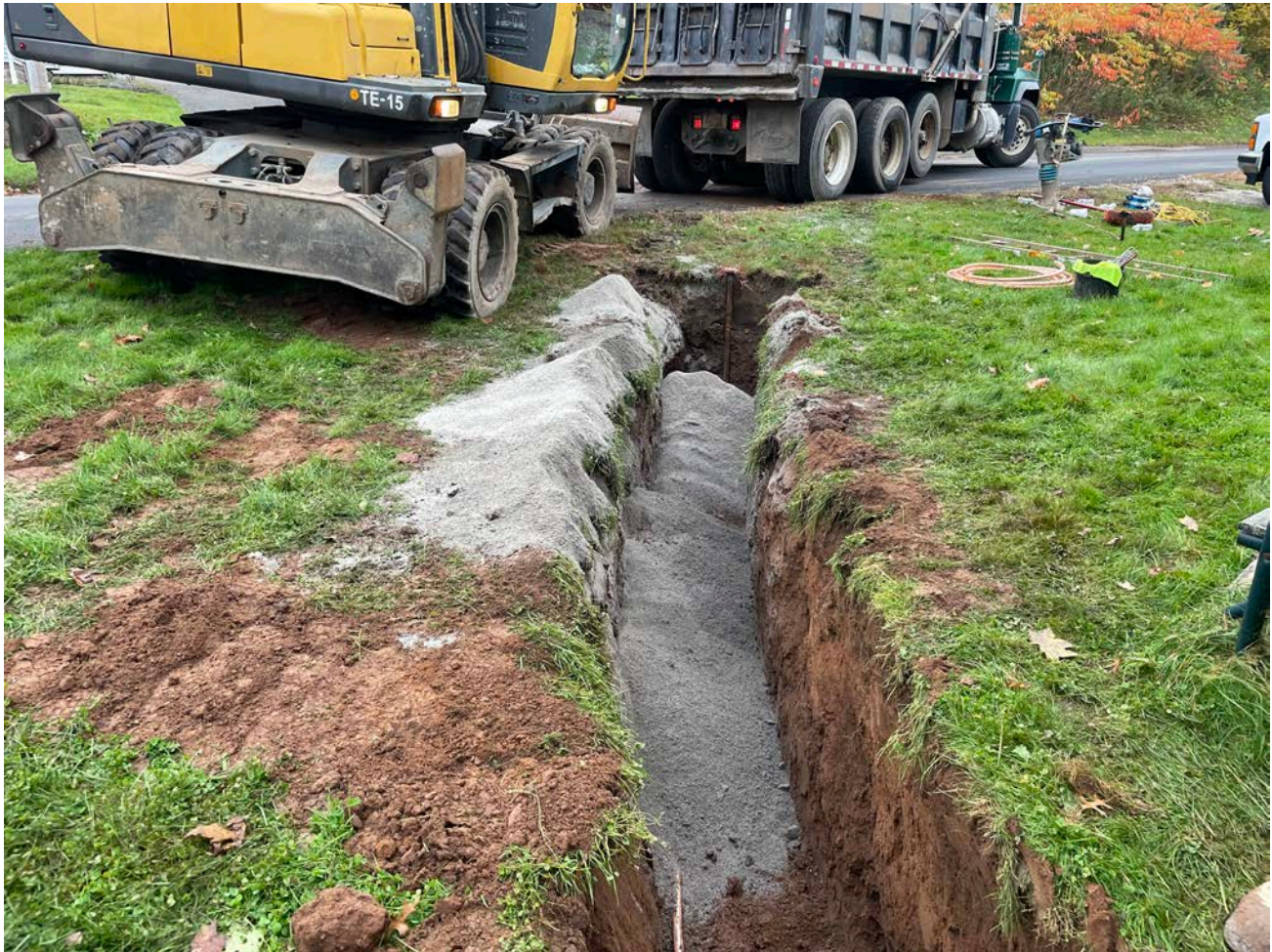
Picture 3: Ludlow saw backfilling over the 1" copper water service line they just installed at the 172 Maple Avenue, Durham, residence. View to the southeast.
