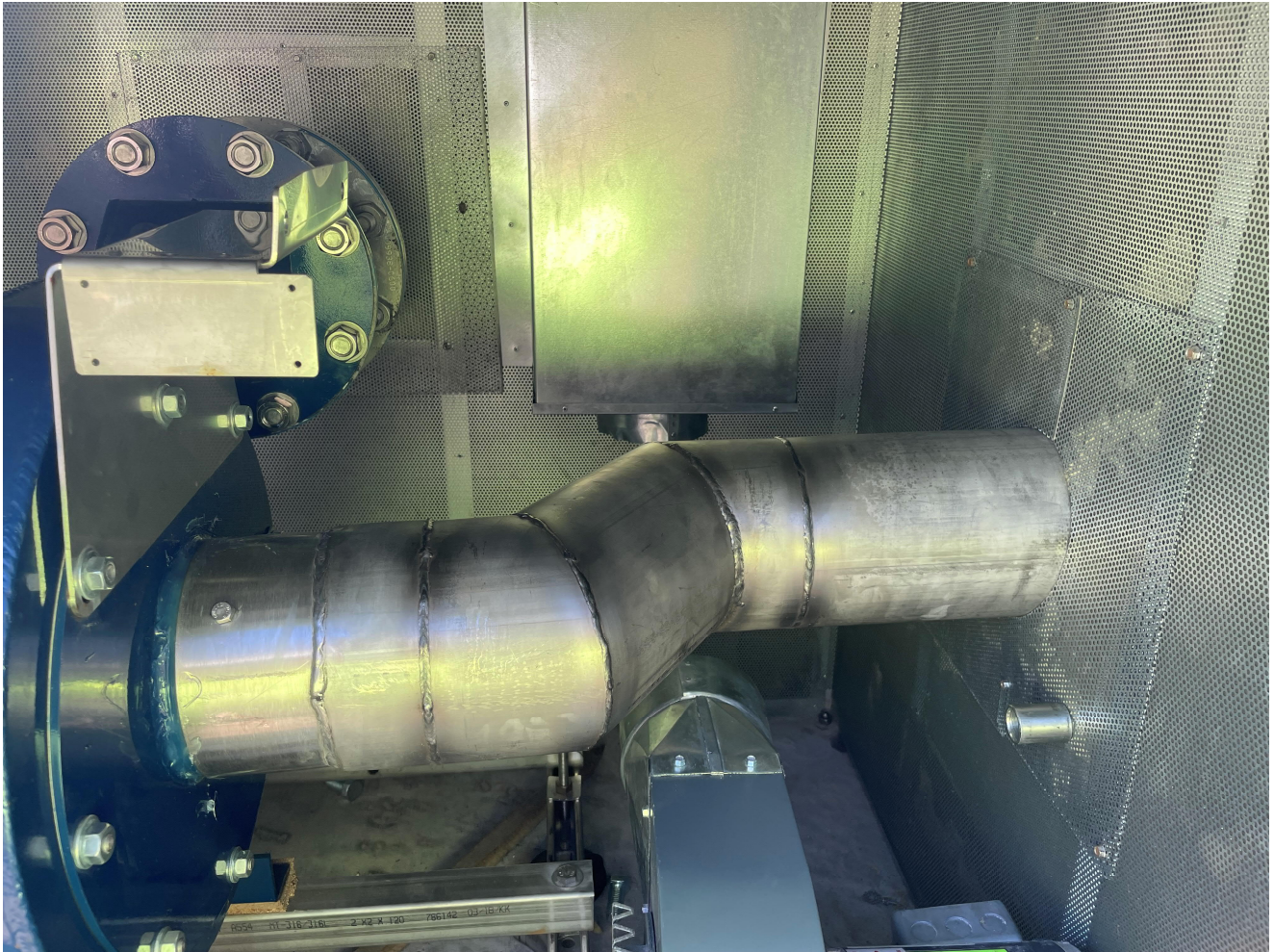
Picture 8: Stainless steel duct that Ludlow's subcontractor fabricated for placement on the blower located inside of the blower cabinet on the northeast side of the water tank. View to the south.
