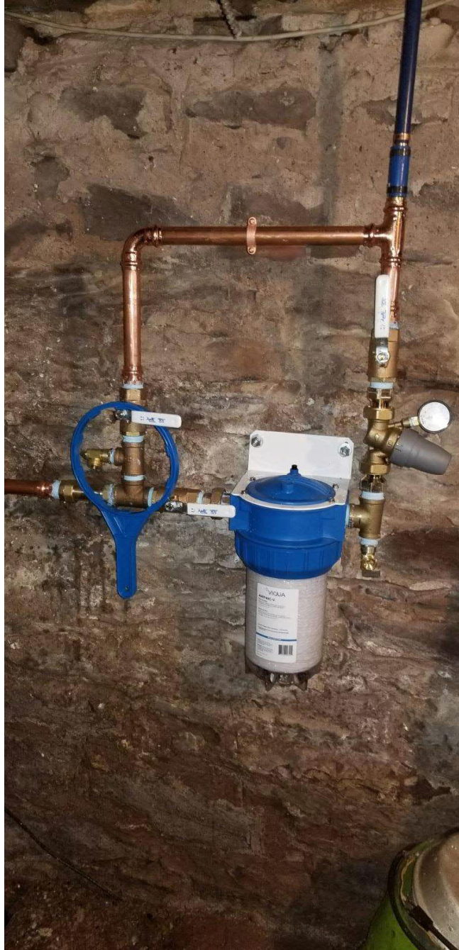
Picture 11: Final water service components that Fazzino Plumbing installed at the 29 Maiden Lane, Durham, residence.
