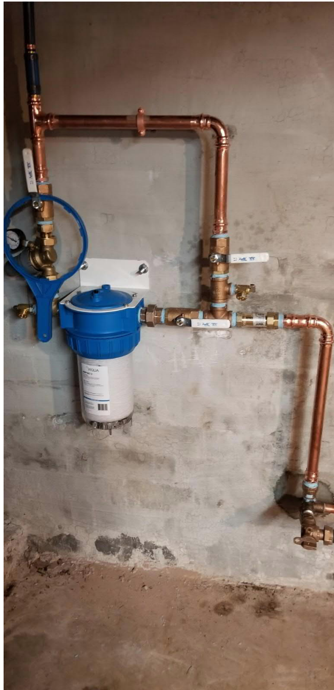
Picture 9: Final water service components that Fazzino Plumbing installed at the 18 Maiden Lane, Durham, residence.
