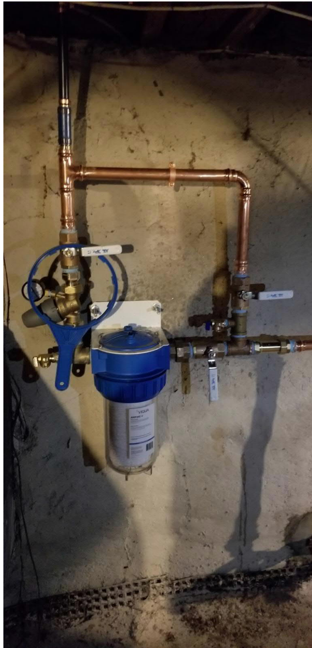
Picture 10: Final water service components that Fazzino Plumbing installed at the 19 Maiden Lane, Durham, residence.
