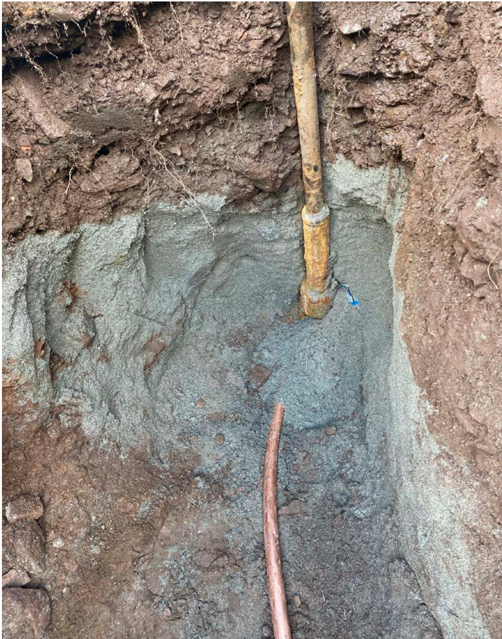
Picture 10: Ludlow connects the 1” copper service to the curb stop for the 19 Maiden Lane residence. View to the North.
