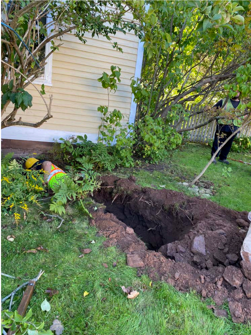
Picture 7: Ludlow excavates a trench for the 1" copper service line down the West side of the house for the 19 Maiden Lane residence in Durham, CT. View to the South.
