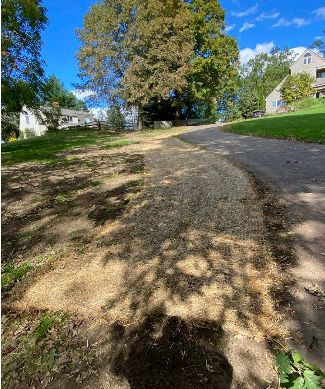
Picture 14: Ludlow restores the portions of the property that were disturbed during the installation of a copper water service line on the 95R Maple Avenue property in Durham CT. Ludlow places seed and hay mats over area for restoration. View to the East.
