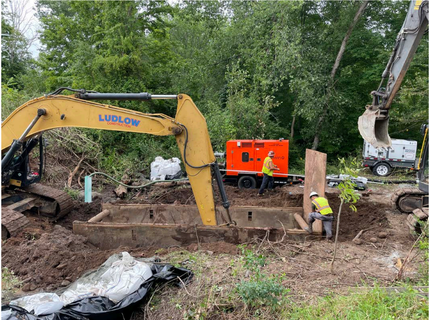
Picture 7: Ludlow excavating silt from within the footprint of a trench box as part of the Maiden Lane stream crossing activities. View to north.
