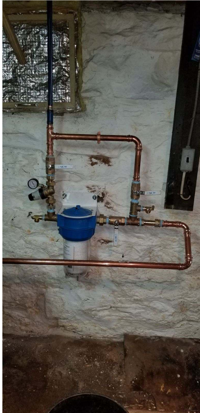
Picture 13: View of final water service components installed at the 322 Main Street residence by Fazzino Plumbing.
