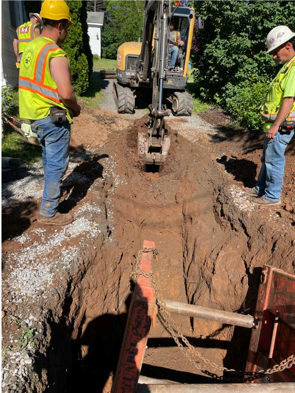
Picture 2: Ludlow excavating for the installation of a 1" copper water service line at the 176 Main Street, Durham, on the northeast corner of the residence. View to the west.
