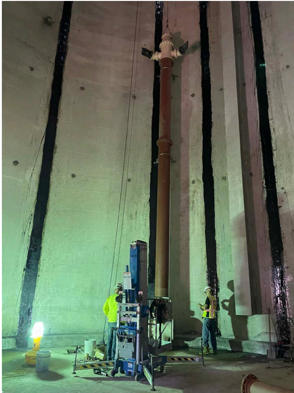
Picture 1: View of the inlet pipe that DN Tanks is in the process of installing inside the water tank located east of the Shared Access Driveway in Middletown. View to the southwest.
