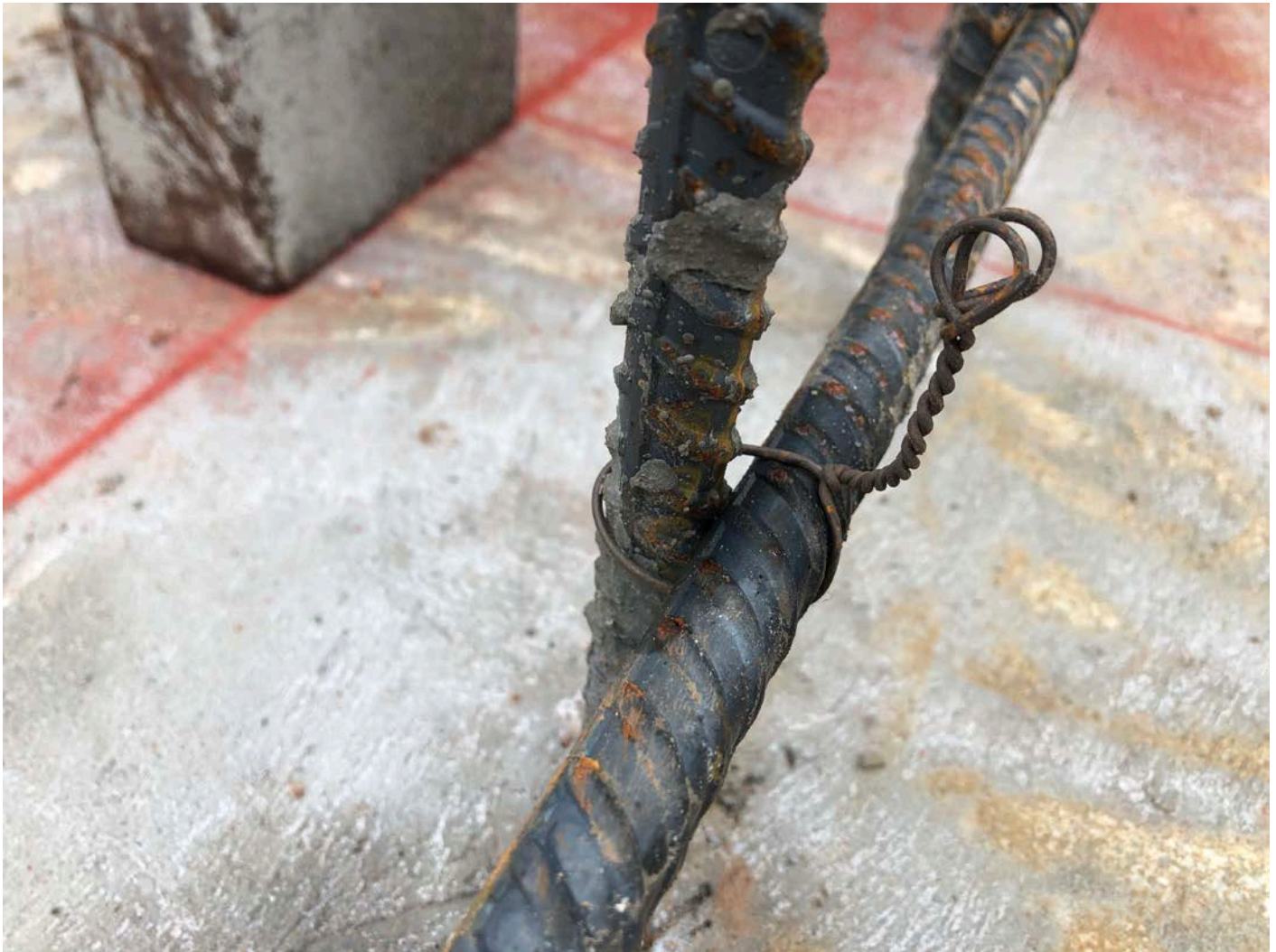
Picture 3: Closeup of intersecting rebar for the frost wall that has been secured with wire ties at the booster station located at Station 750+63 in Middletown.
