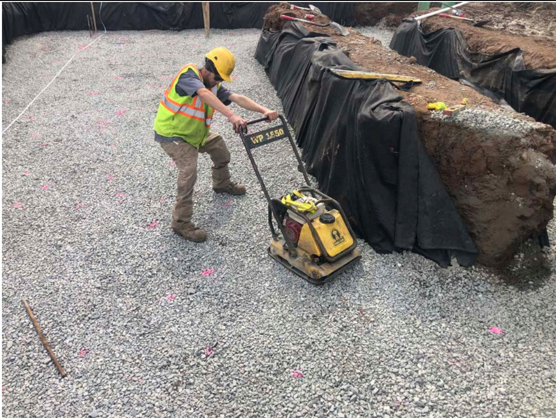
Picture 1: Ludlow compacting ¾" gravel on the booster station footprint at Station 750+63 in Middletown. View to the east.
