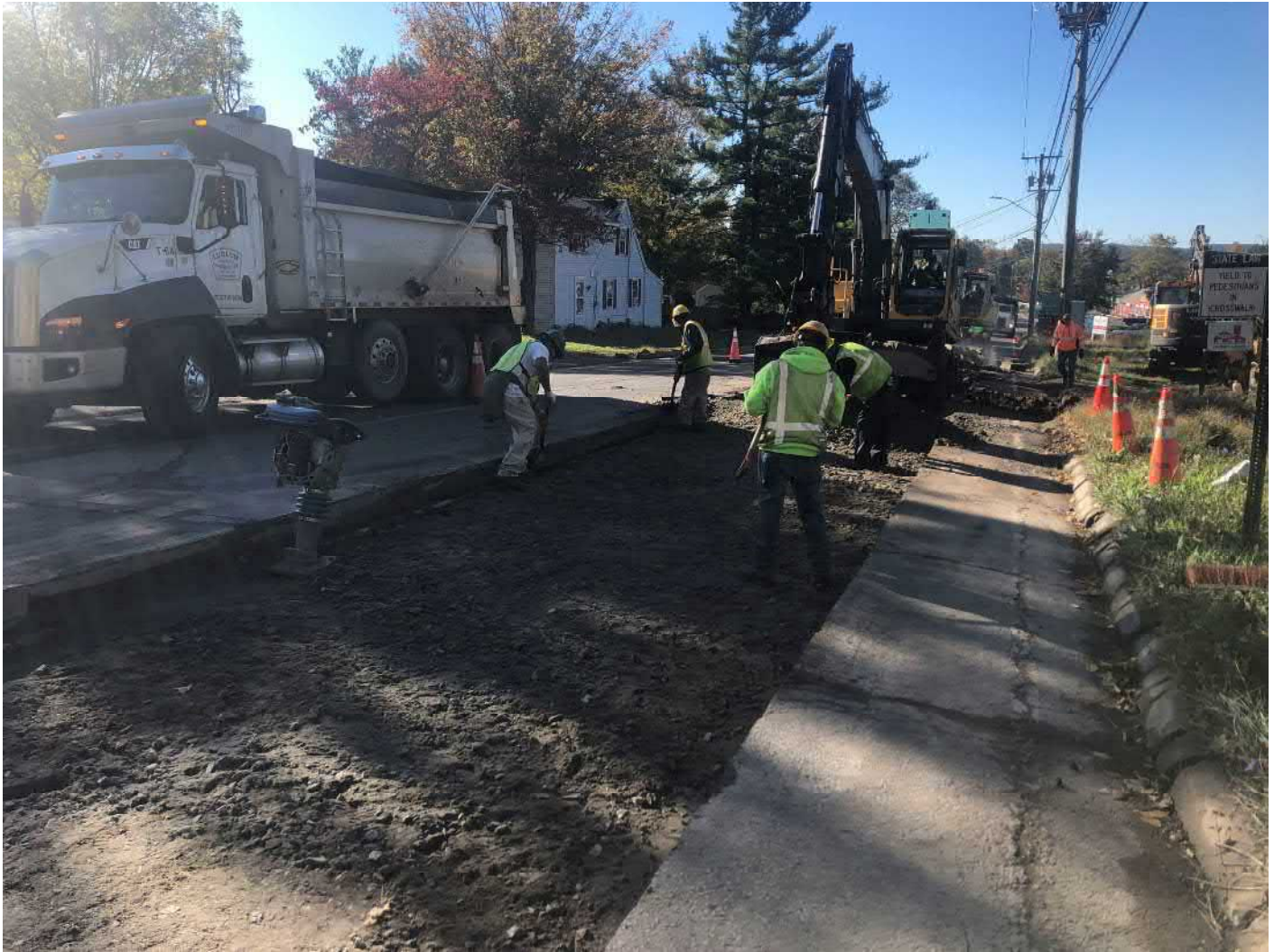
Picture 1: Ludlow stripping back asphalt and compacting 1.5" processed gravel as they prepare to place permanent paving on the southbound lane of Main Street, Durham. View to the south.
