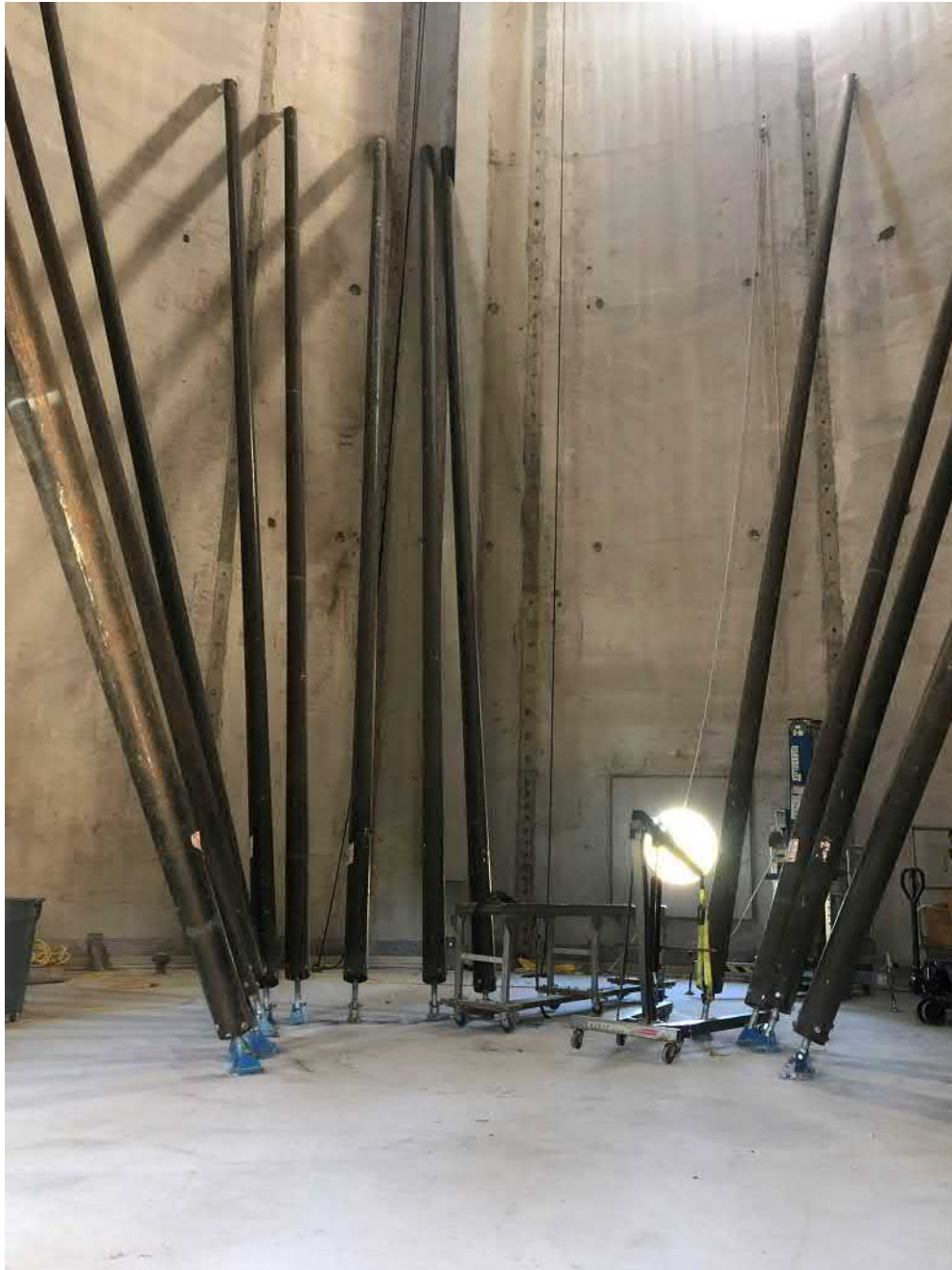
Picture 8: Knee braces inside of the water tank that are being removed today. Water tank work zone located to the east of the Shared Access Driveway, Middletown. View to the west.
