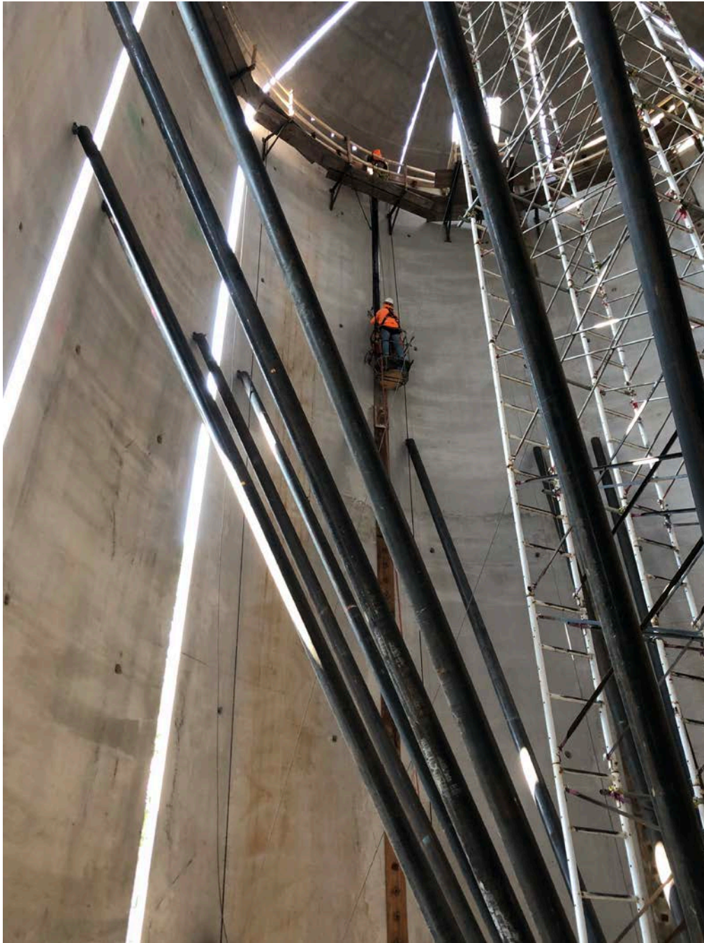
Picture 3: DN Tanks in the process of bolting plywood to the back of a slot panel from the inside of the water tank. Water tank work zone, east of the Shared Access Driveway, Middletown.
