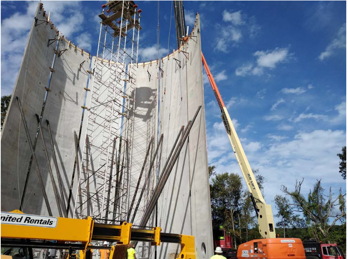
Picture 22: Removing lifting cables from sixth tank wall panel and securing to adjacent panels. Shared access driveway, Middletown; view to the northeast.
