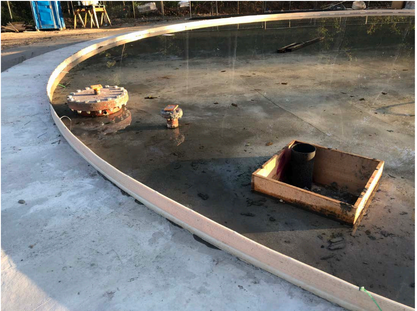
Picture 1: View of PVC water stop and the 3 pipes entering the water tank. Water tank work zone, east of the Shared Access Driveway, Middletown. View to the northwest.
