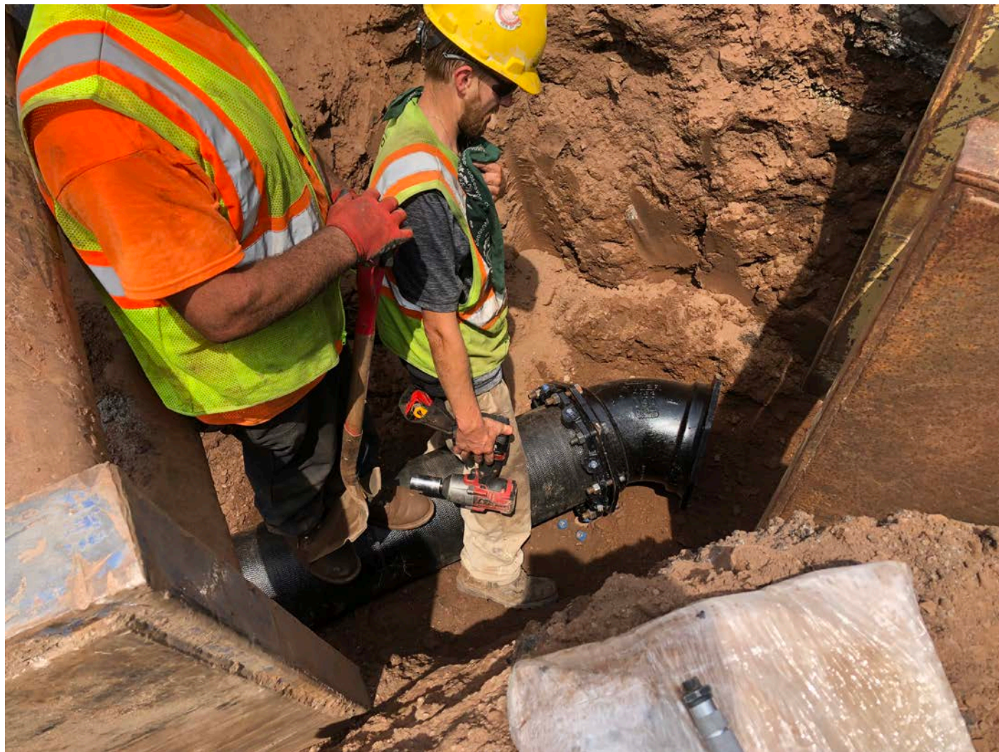
Picture 5: Ludlow installing 45° bend at Station 906+38, just north of the Maple Avenue stream crossing. View to the north.
