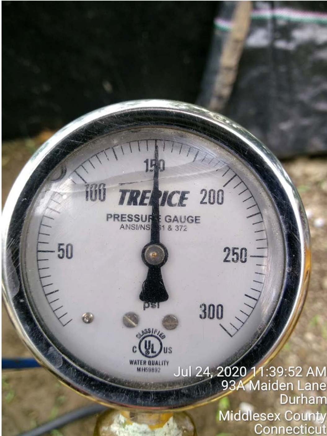
Picture 11: End pressure on the test performed on the Maiden Lane water line from a gate valve at Station 412+14 and gate valve at the intersection of Maiden Lane and Pickett Lane.
