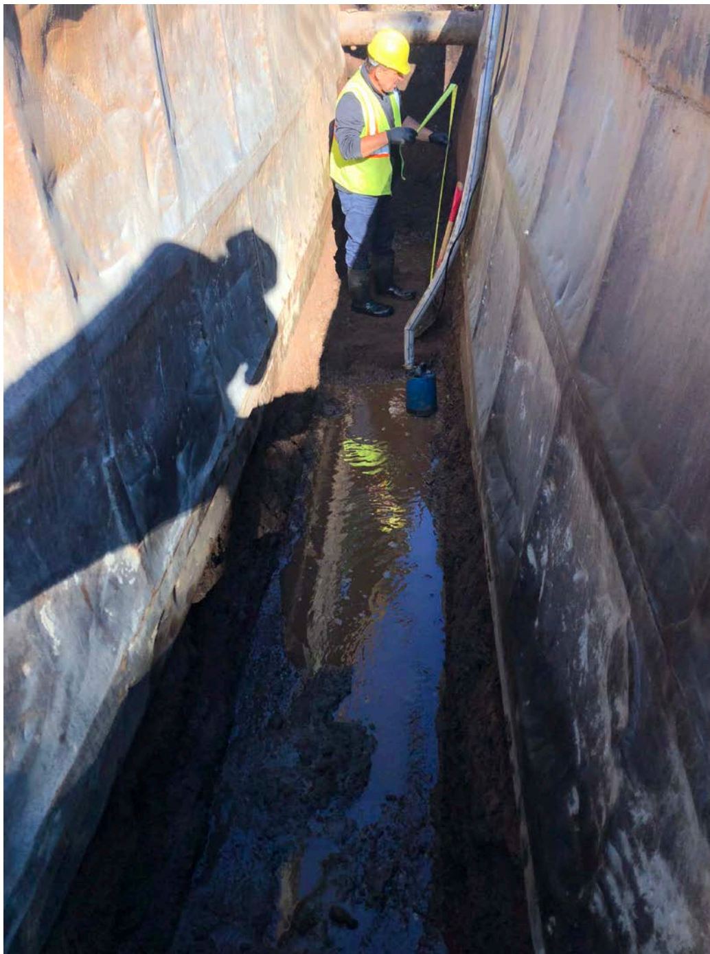
Picture 2: Ludlow setting up pump water out of the trench at ~Station 425+90 on Maiden Lane. View to the west.
