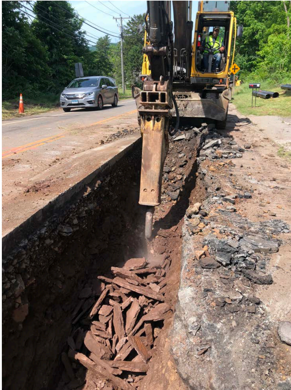
Picture 4: Ludlow hammering rock in order to place 12" DIP at proper depth. Route 68, Durham. View to the west.
