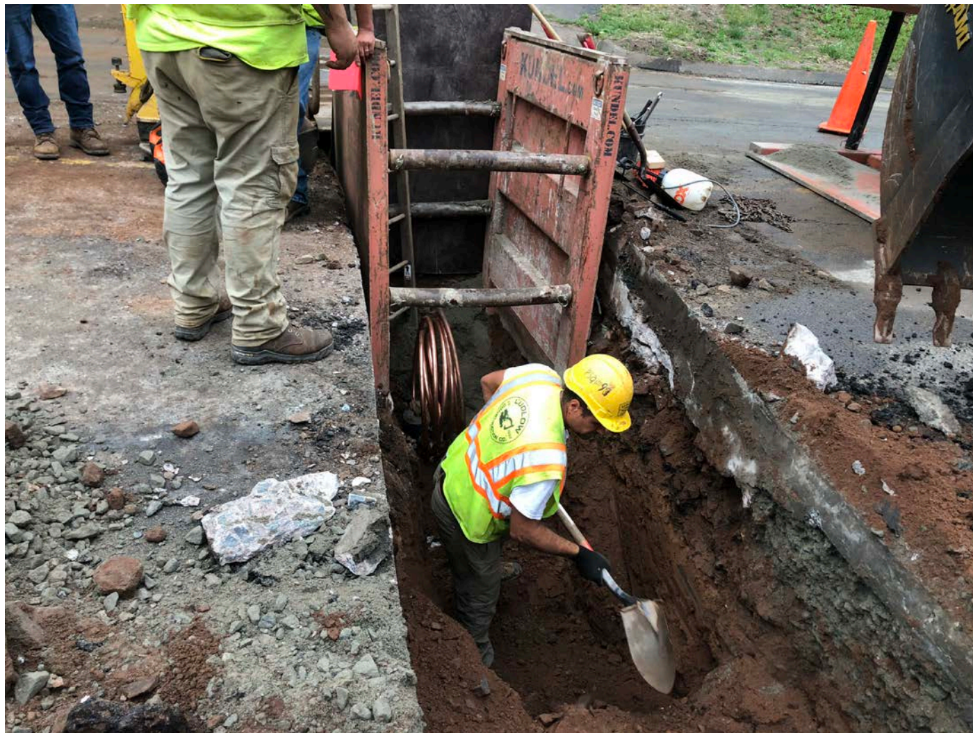
Picture 3: Ludlow installing 1" copper line for curb stop at Station 143+34. Main Street, Durham. View to the east.
