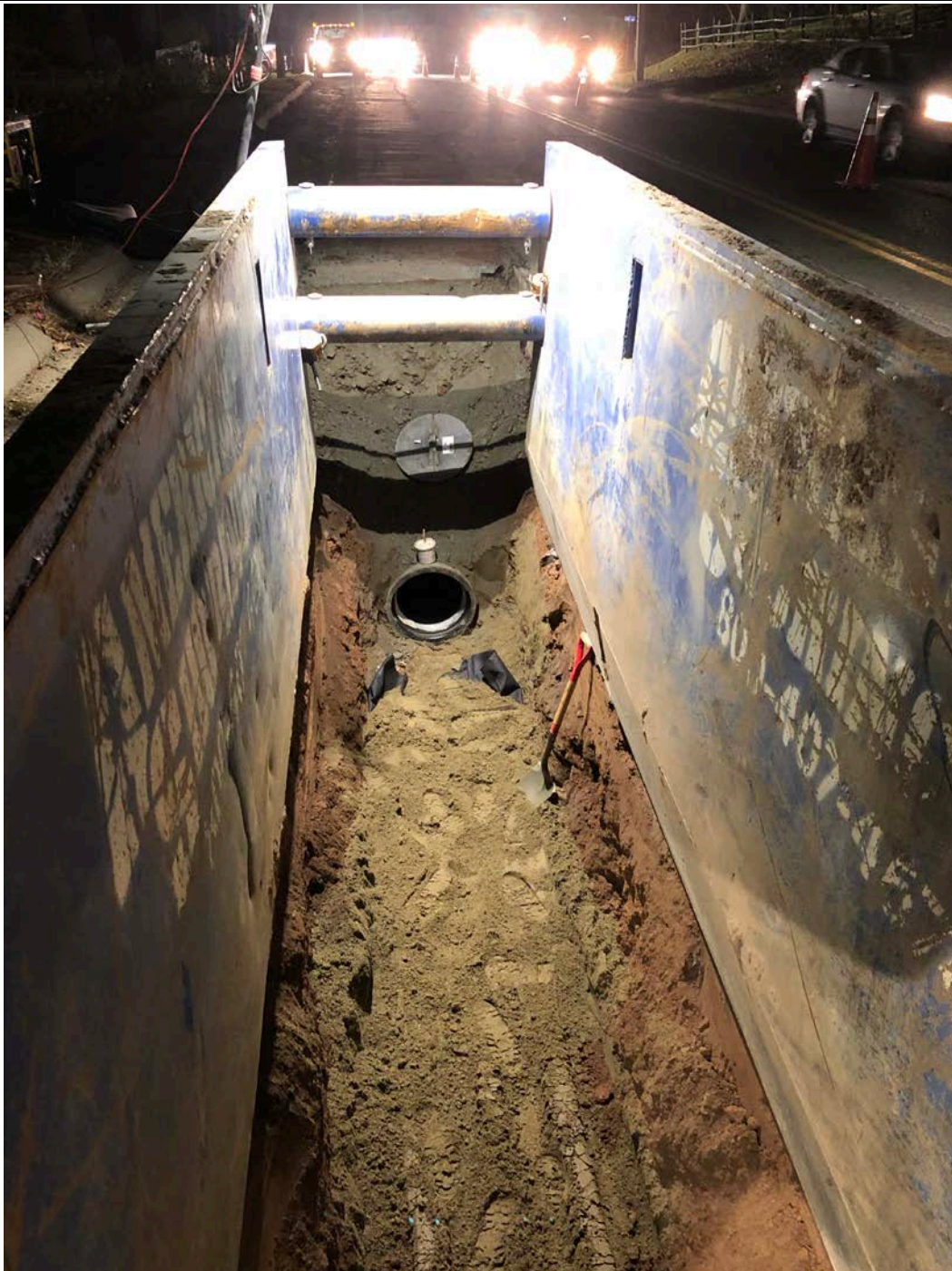
Figure 1 – End of water main at Sta. 143+17, ready to place 1 st pipe section
