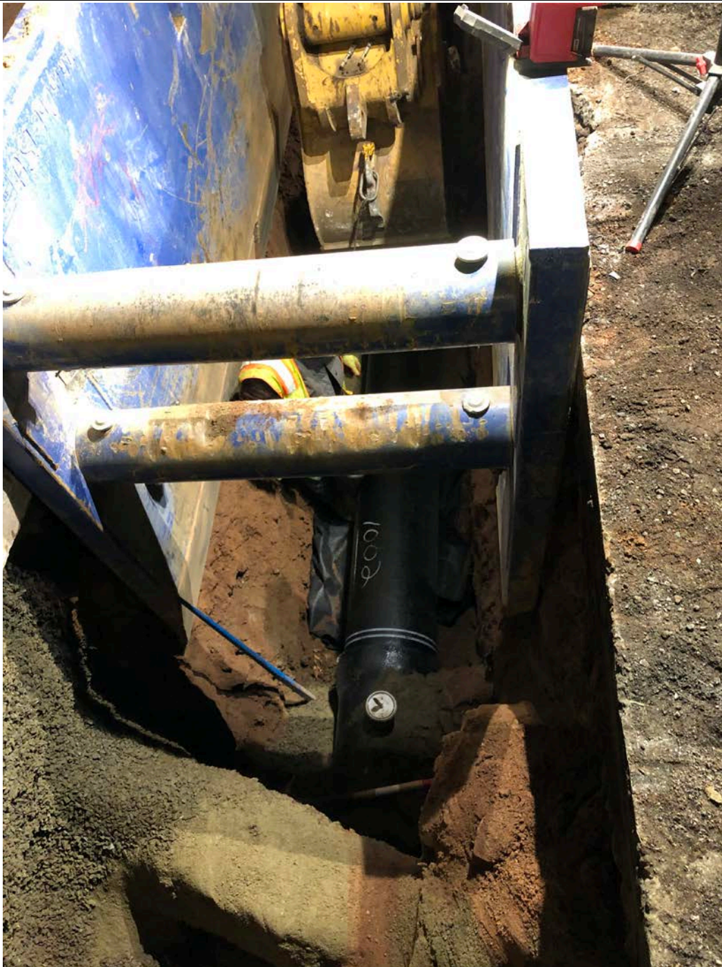
Figure 4 – Attaching 6 th pipe section, 5 th section passes under storm drain seen at bottom of picture
