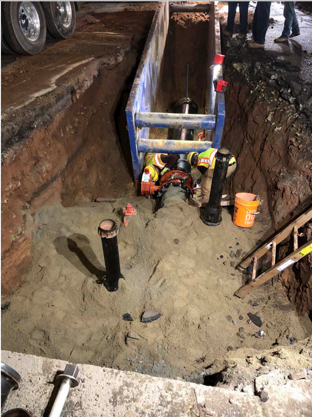
Figure 3 – Attaching 1 st pipe section to valve section, pipe bedding partially laid
