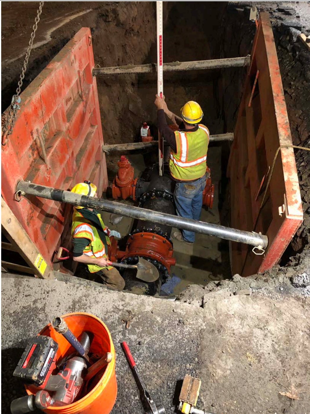
Figure 2 – Taking survey point of placed valve section in trench
