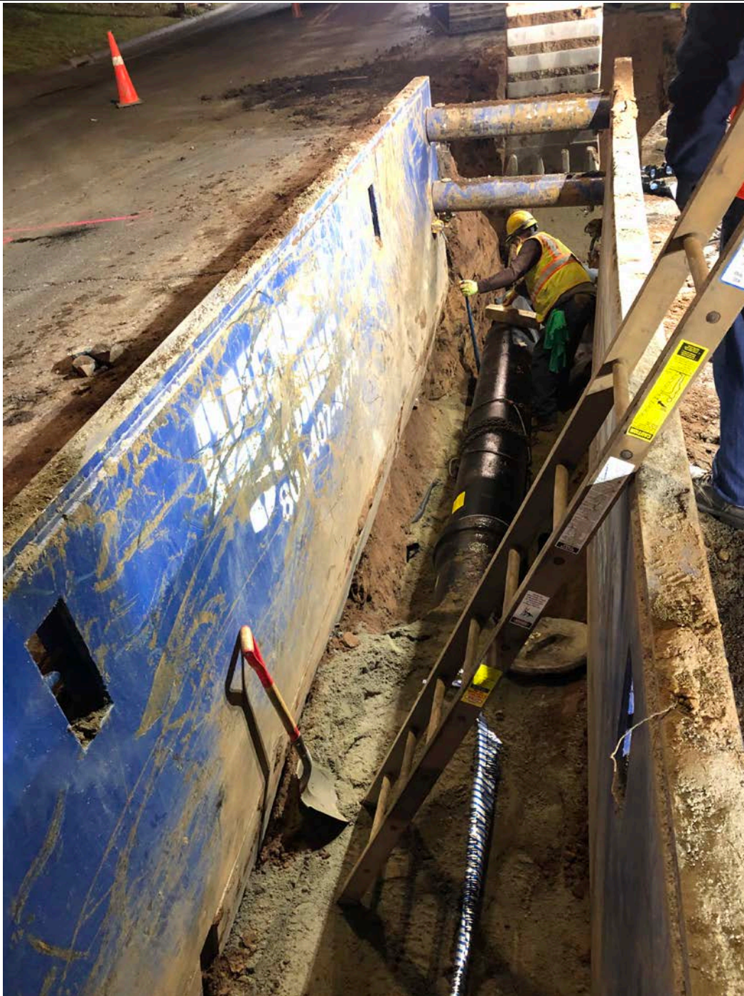
Figure 5 – Placing 8 th pipe section
