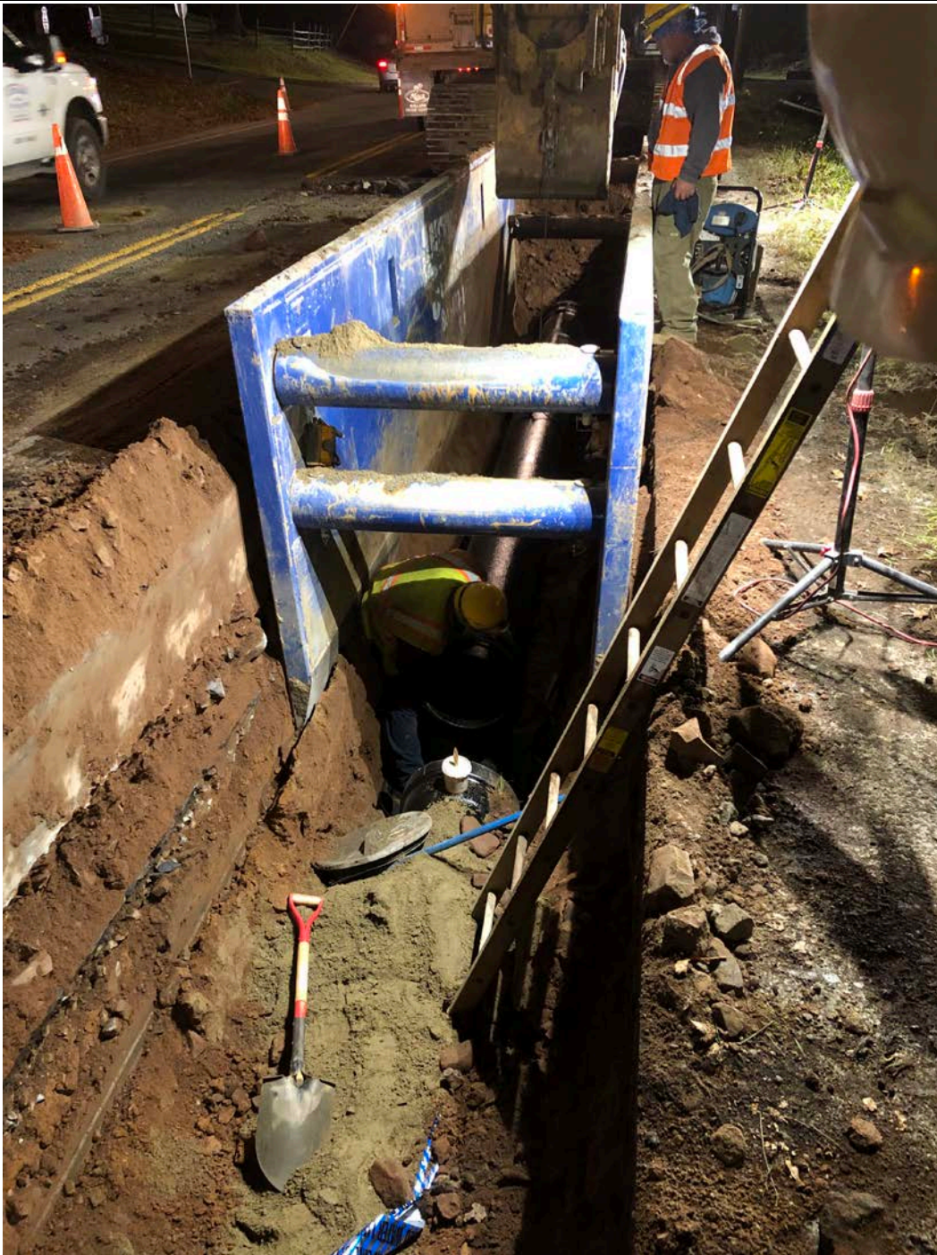
Figure 1 – Placing 3 rd pipe section
