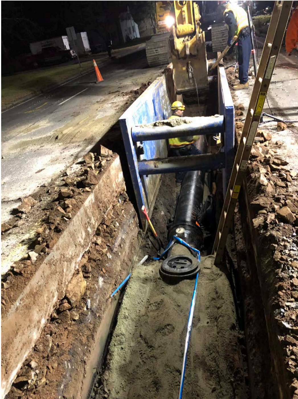
Figure 5 – Placing 5 th pipe section
