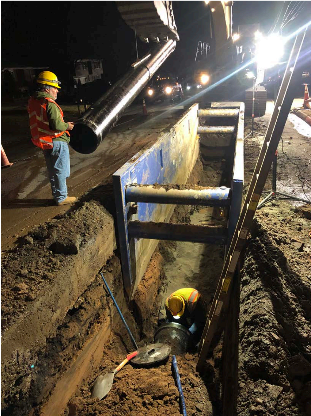
Figure 1 – Preparing to place 2 nd pipe section
