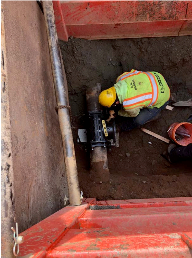
Figure 5 – Ludlow levels, blocks, and shims the new tapping sleeve fitting.
